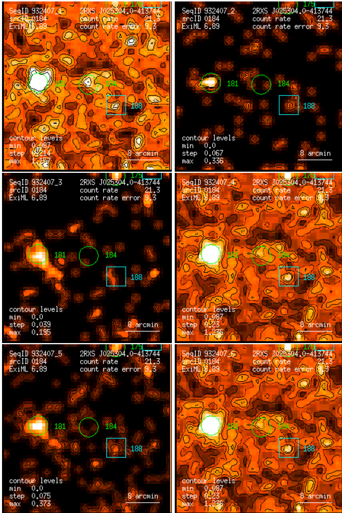
Figure 184: RASS 932407: detection 0184: band rate images, Gaussian filter: (1) PSPC channels 11 – 41, (2) 52 – 90, (3) 91 – 201, (4) 11 – 235, (5) 52 – 201, (6) 11 – 201. Broad band rates in counts/ks. Band rate contour levels in counts/ks/arcmin 2 .
