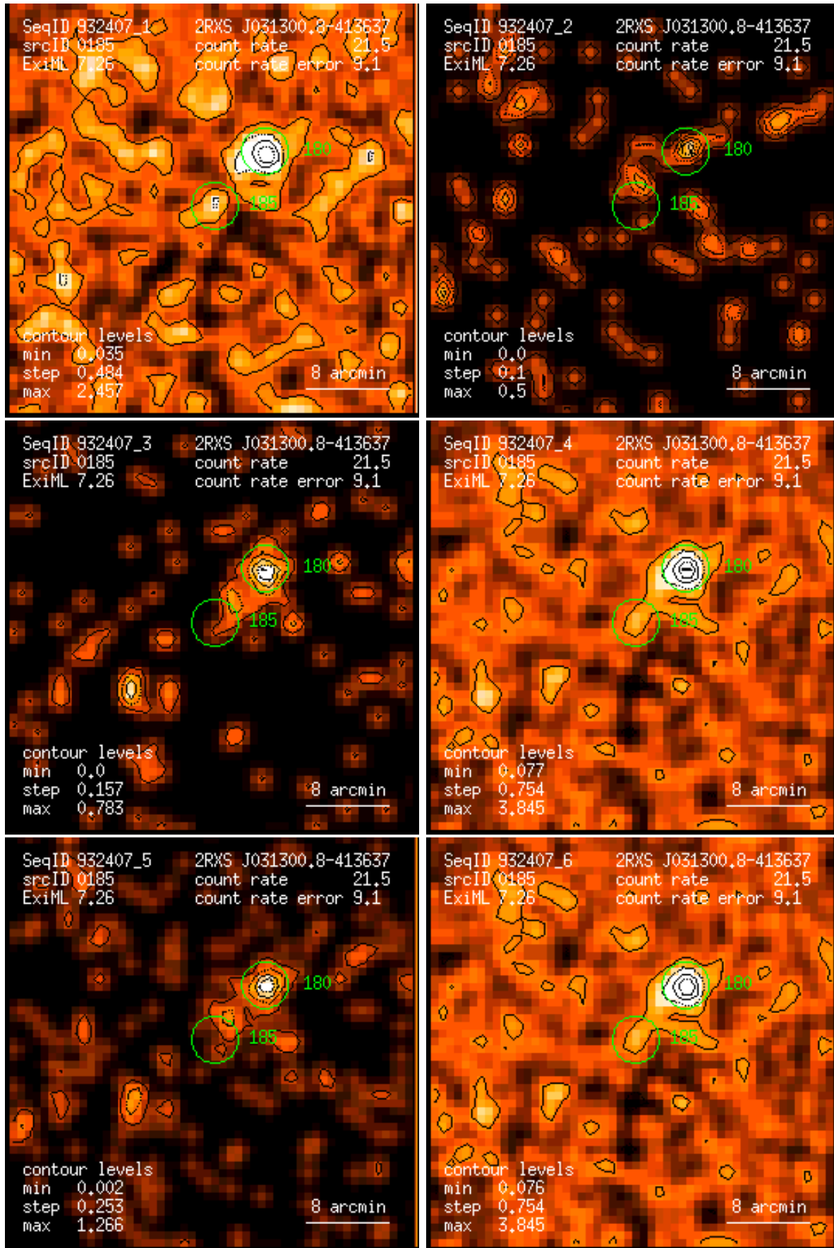
Figure 185: RASS 932407: detection 0185: band rate images, Gaussian filter: (1) PSPC channels 11 – 41, (2) 52 – 90, (3) 91 – 201, (4) 11 – 235, (5) 52 – 201, (6) 11 – 201. Broad band rates in counts/ks. Band rate contour levels in counts/ks/arcmin 2 .
