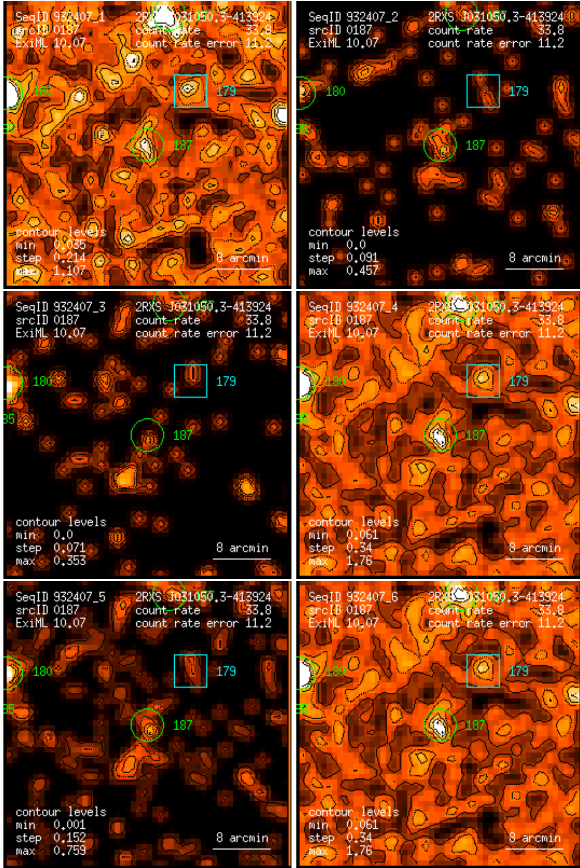
Figure 187: RASS 932407: detection 0187: band rate images, Gaussian filter: (1) PSPC channels 11 – 41, (2) 52 – 90, (3) 91 – 201, (4) 11 – 235, (5) 52 – 201, (6) 11 – 201. Broad band rates in counts/ks. Band rate contour levels in counts/ks/arcmin 2 .
