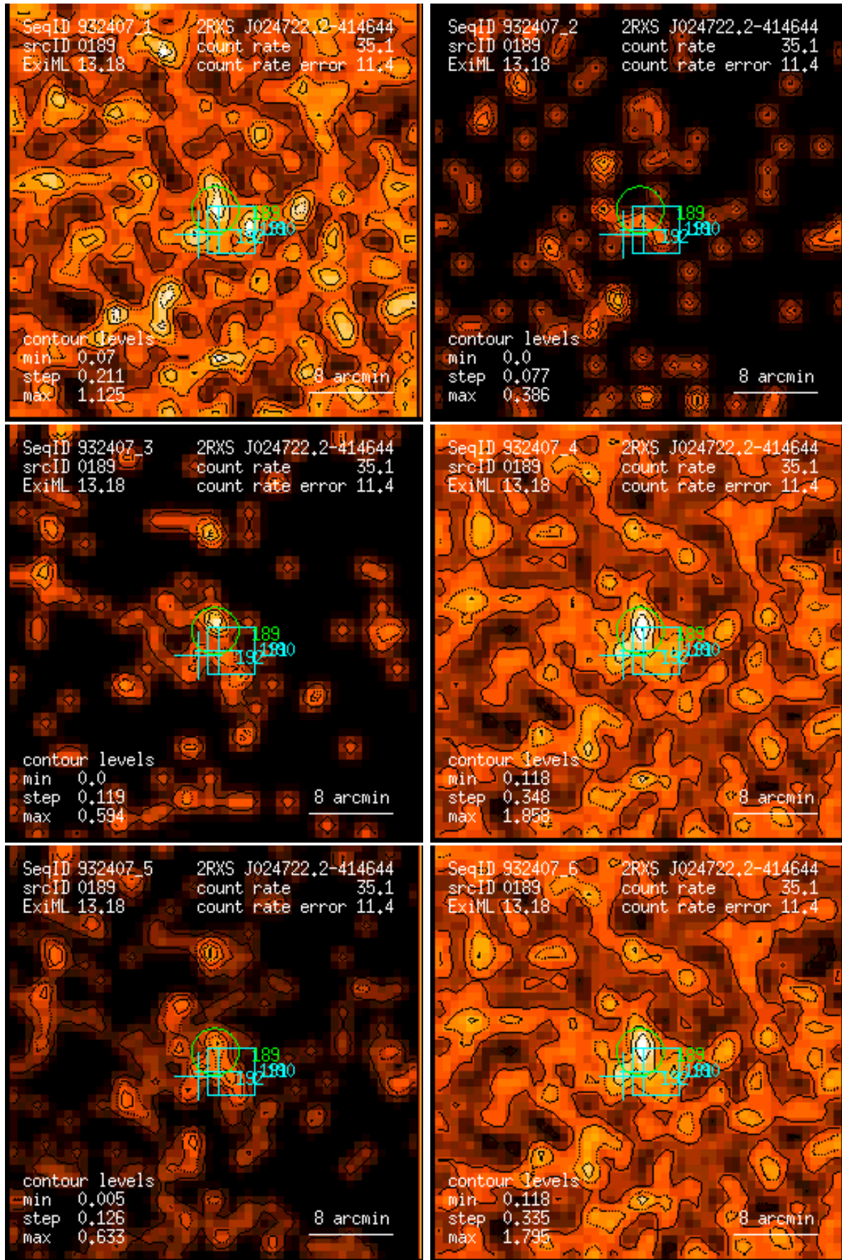
Figure 189: RASS 932407: detection 0189: band rate images, Gaussian filter: (1) PSPC channels 11 – 41, (2) 52 – 90, (3) 91 – 201, (4) 11 – 235, (5) 52 – 201, (6) 11 – 201. Broad band rates in counts/ks. Band rate contour levels in counts/ks/arcmin 2 .
