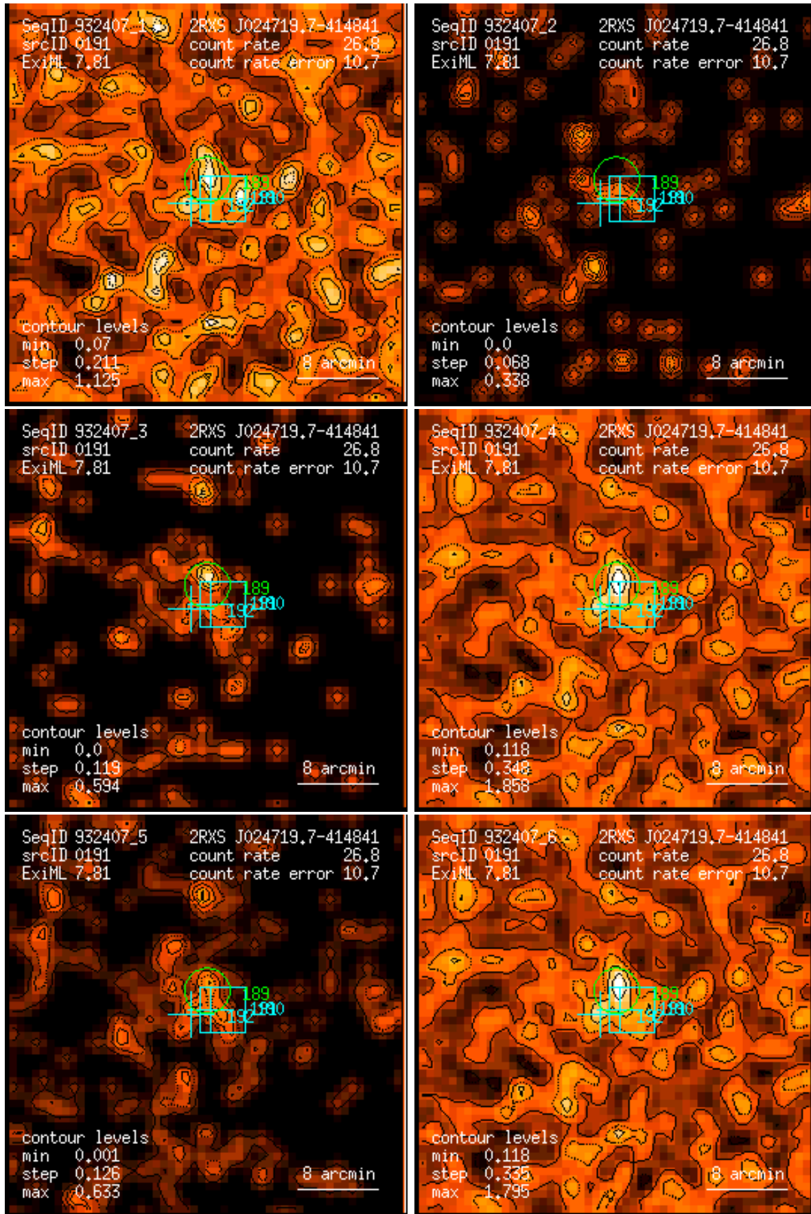
Figure 191: RASS 932407: detection 0191: band rate images, Gaussian filter: (1) PSPC channels 11 – 41, (2) 52 – 90, (3) 91 – 201, (4) 11 – 235, (5) 52 – 201, (6) 11 – 201. Broad band rates in counts/ks. Band rate contour levels in counts/ks/arcmin 2 .
