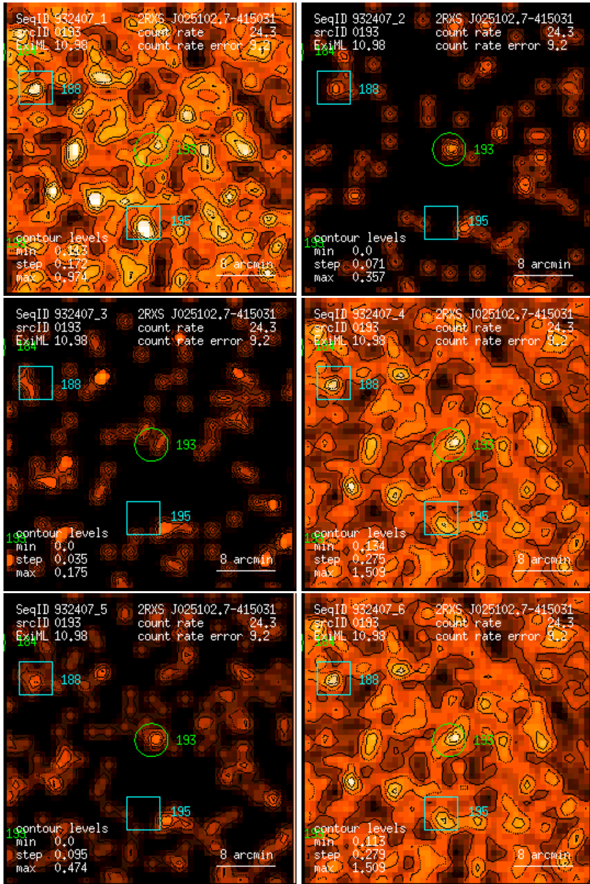
Figure 193: RASS 932407: detection 0193: band rate images, Gaussian filter: (1) PSPC channels 11 – 41, (2) 52 – 90, (3) 91 – 201, (4) 11 – 235, (5) 52 – 201, (6) 11 – 201. Broad band rates in counts/ks. Band rate contour levels in counts/ks/arcmin 2 .
