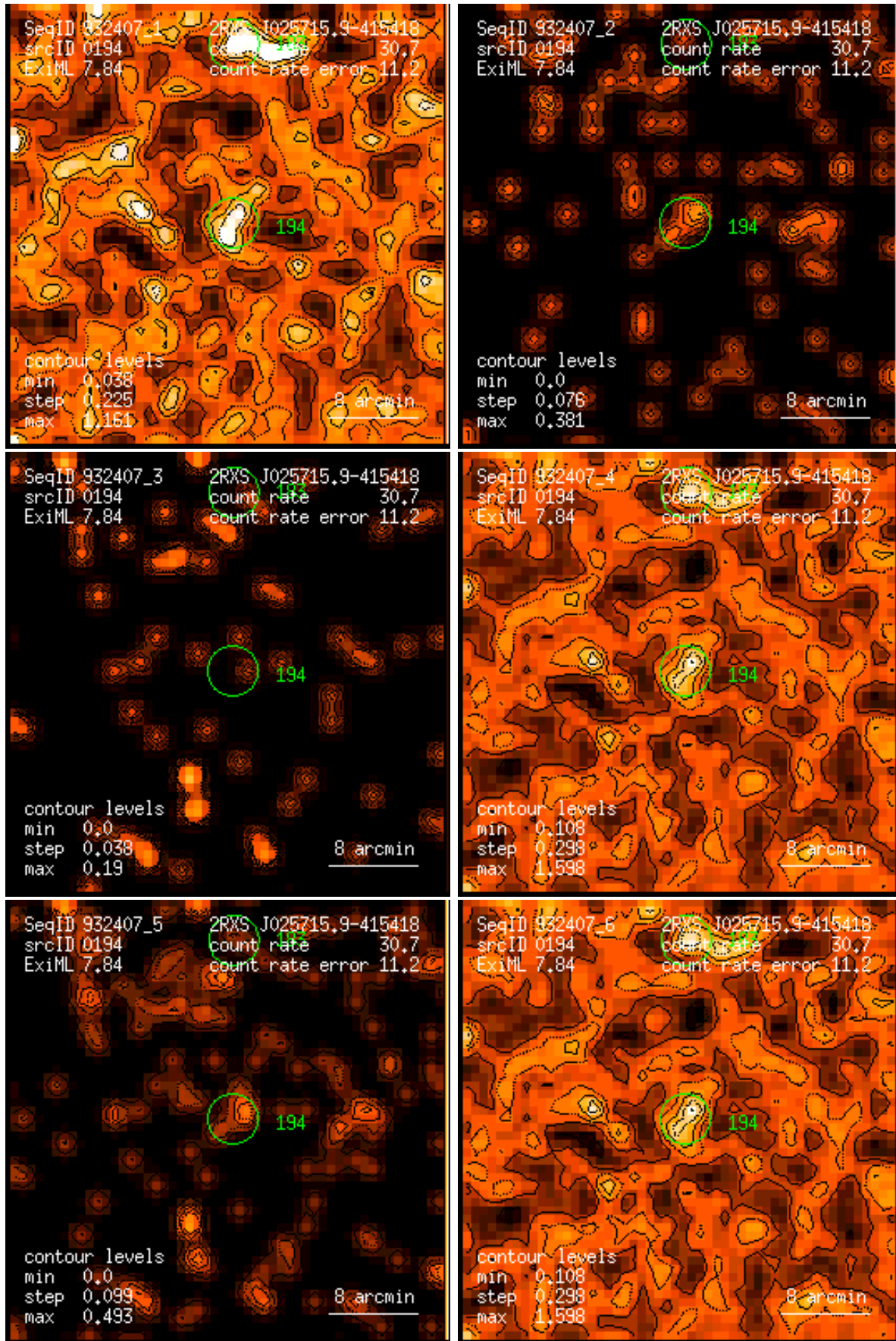
Figure 194: RASS 932407: detection 0194: band rate images, Gaussian filter: (1) PSPC channels 11 – 41, (2) 52 – 90, (3) 91 – 201, (4) 11 – 235, (5) 52 – 201, (6) 11 – 201. Broad band rates in counts/ks. Band rate contour levels in counts/ks/arcmin 2 .
