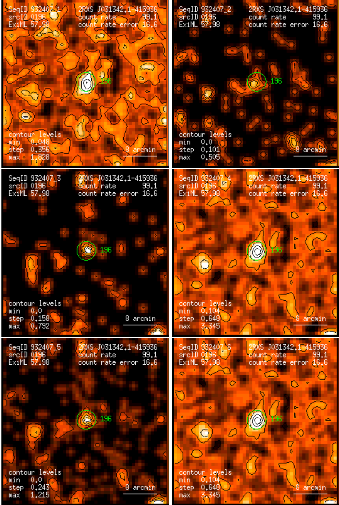
Figure 196: RASS 932407: detection 0196: band rate images, Gaussian filter: (1) PSPC channels 11 – 41, (2) 52 – 90, (3) 91 – 201, (4) 11 – 235, (5) 52 – 201, (6) 11 – 201. Broad band rates in counts/ks. Band rate contour levels in counts/ks/arcmin 2 .
