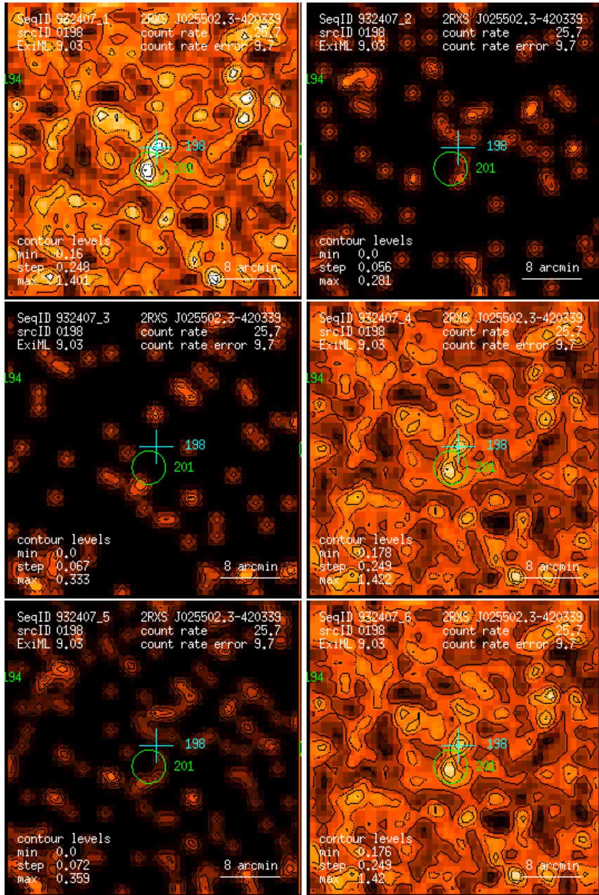
Figure 198: RASS 932407: detection 0198: band rate images, Gaussian filter: (1) PSPC channels 11 – 41, (2) 52 – 90, (3) 91 – 201, (4) 11 – 235, (5) 52 – 201, (6) 11 – 201. Broad band rates in counts/ks. Band rate contour levels in counts/ks/arcmin 2 .
