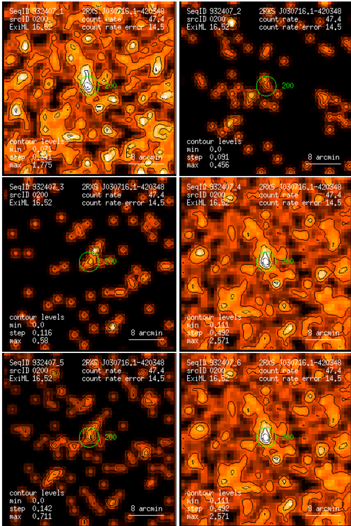
Figure 200: RASS 932407: detection 0200: band rate images, Gaussian filter: (1) PSPC channels 11 – 41, (2) 52 – 90, (3) 91 – 201, (4) 11 – 235, (5) 52 – 201, (6) 11 – 201. Broad band rates in counts/ks. Band rate contour levels in counts/ks/arcmin 2 .
