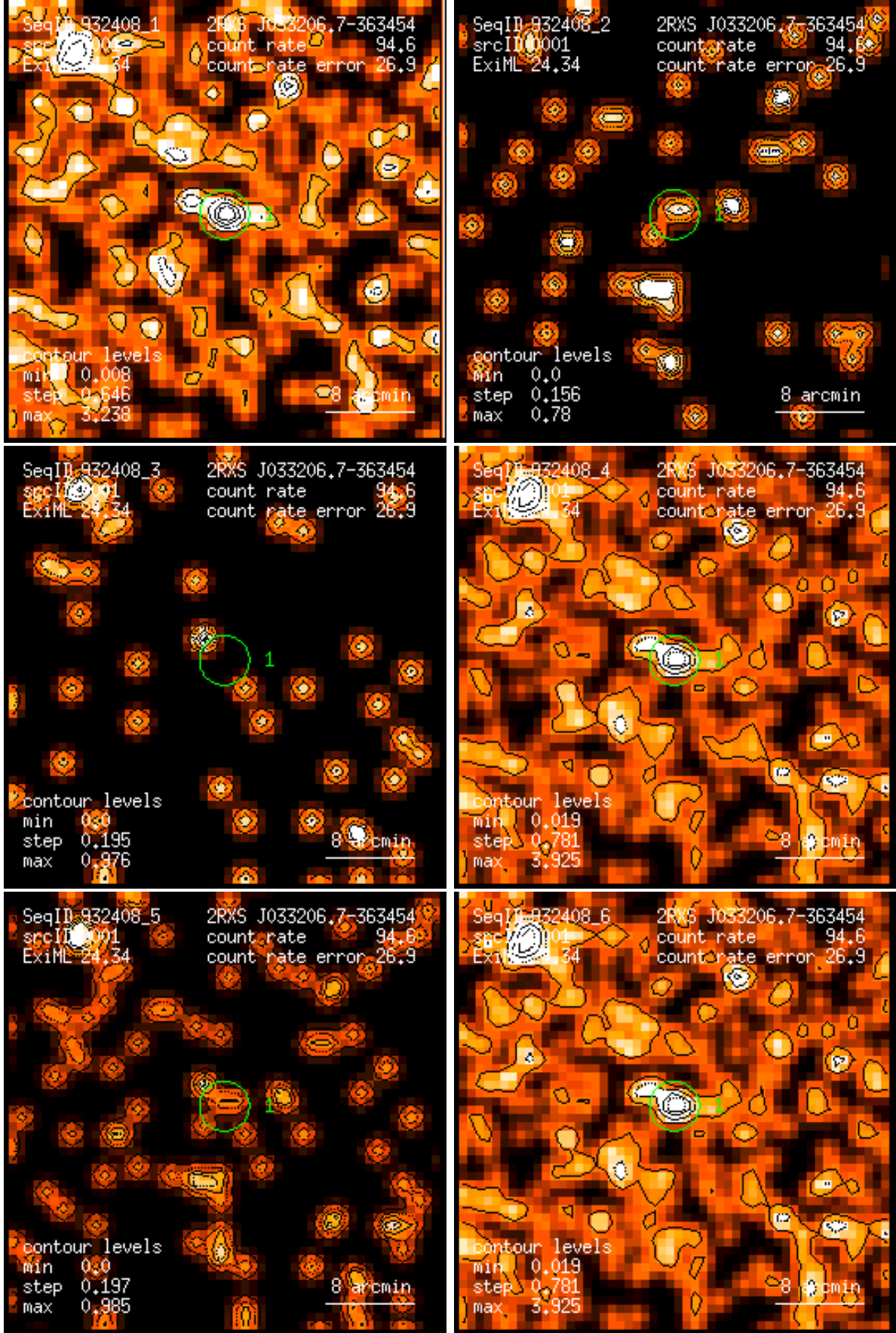
Figure 1: RASS 932408: detection 0001: band rate images, Gaussian filter: (1) PSPC channels 11 – 41, (2) 52 – 90, (3) 91 – 201, (4) 11 – 235, (5) 52 – 201, (6) 11 – 201. Broad band rates in counts/ks. Band rate contour levels in counts/ks/arcmin 2 .
