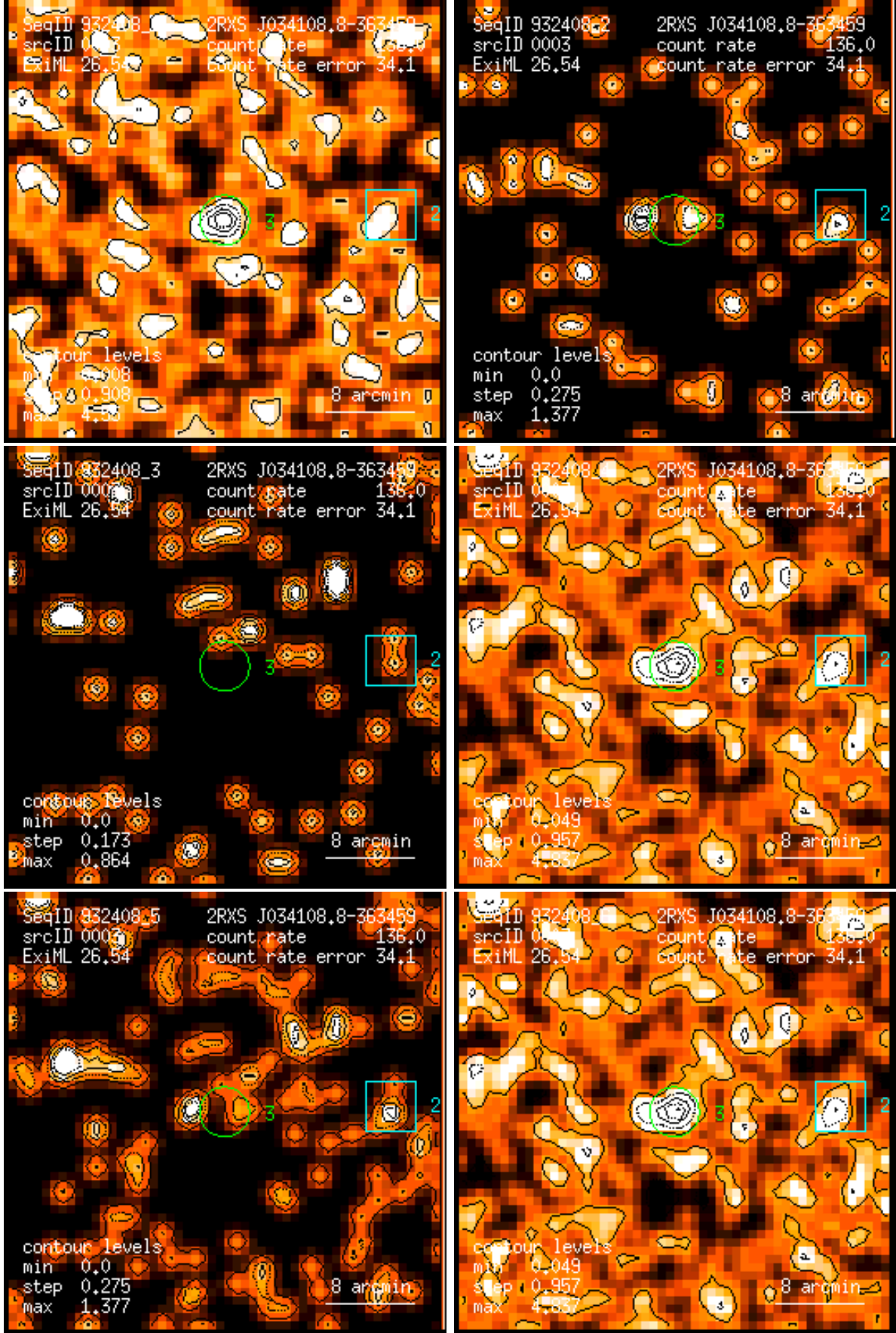
Figure 3: RASS 932408: detection 0003: band rate images, Gaussian filter: (1) PSPC channels 11 – 41, (2) 52 – 90, (3) 91 – 201, (4) 11 – 235, (5) 52 – 201, (6) 11 – 201. Broad band rates in counts/ks. Band rate contour levels in counts/ks/arcmin 2 .
