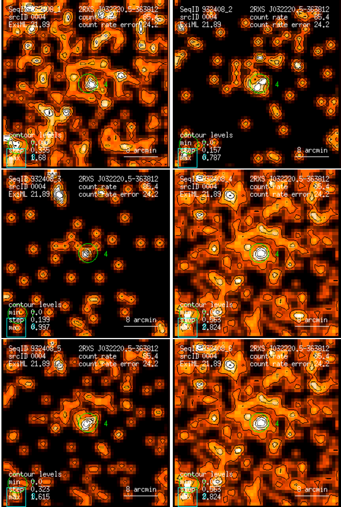
Figure 4: RASS 932408: detection 0004: band rate images, Gaussian filter: (1) PSPC channels 11 – 41, (2) 52 – 90, (3) 91 – 201, (4) 11 – 235, (5) 52 – 201, (6) 11 – 201. Broad band rates in counts/ks. Band rate contour levels in counts/ks/arcmin 2 .
