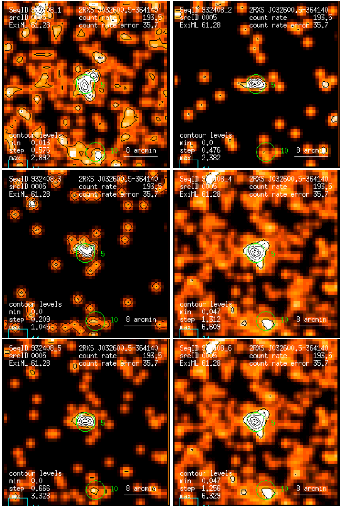
Figure 5: RASS 932408: detection 0005: band rate images, Gaussian filter: (1) PSPC channels 11 – 41, (2) 52 – 90, (3) 91 – 201, (4) 11 – 235, (5) 52 – 201, (6) 11 – 201. Broad band rates in counts/ks. Band rate contour levels in counts/ks/arcmin 2 .
