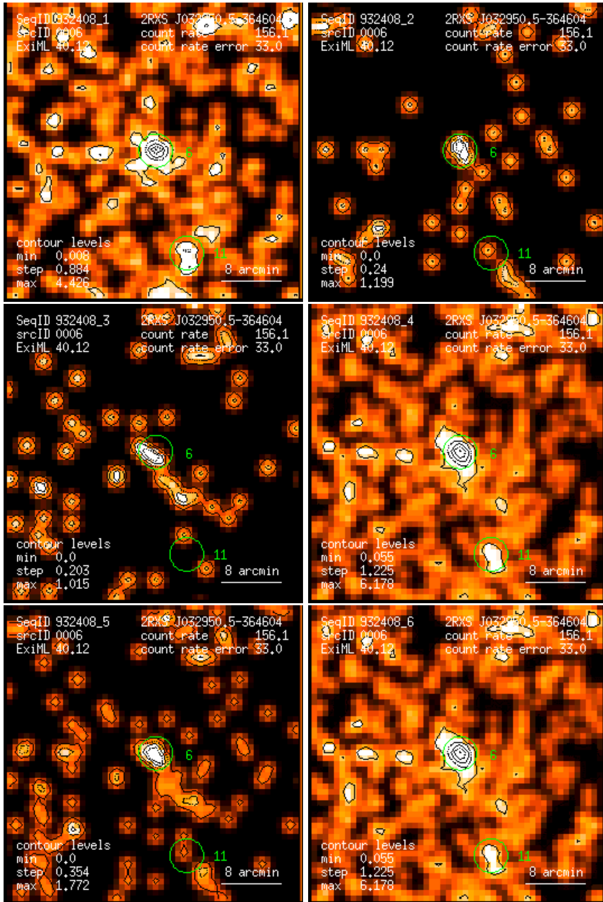
Figure 6: RASS 932408: detection 0006: band rate images, Gaussian filter: (1) PSPC channels 11 – 41, (2) 52 – 90, (3) 91 – 201, (4) 11 – 235, (5) 52 – 201, (6) 11 – 201. Broad band rates in counts/ks. Band rate contour levels in counts/ks/arcmin 2 .
