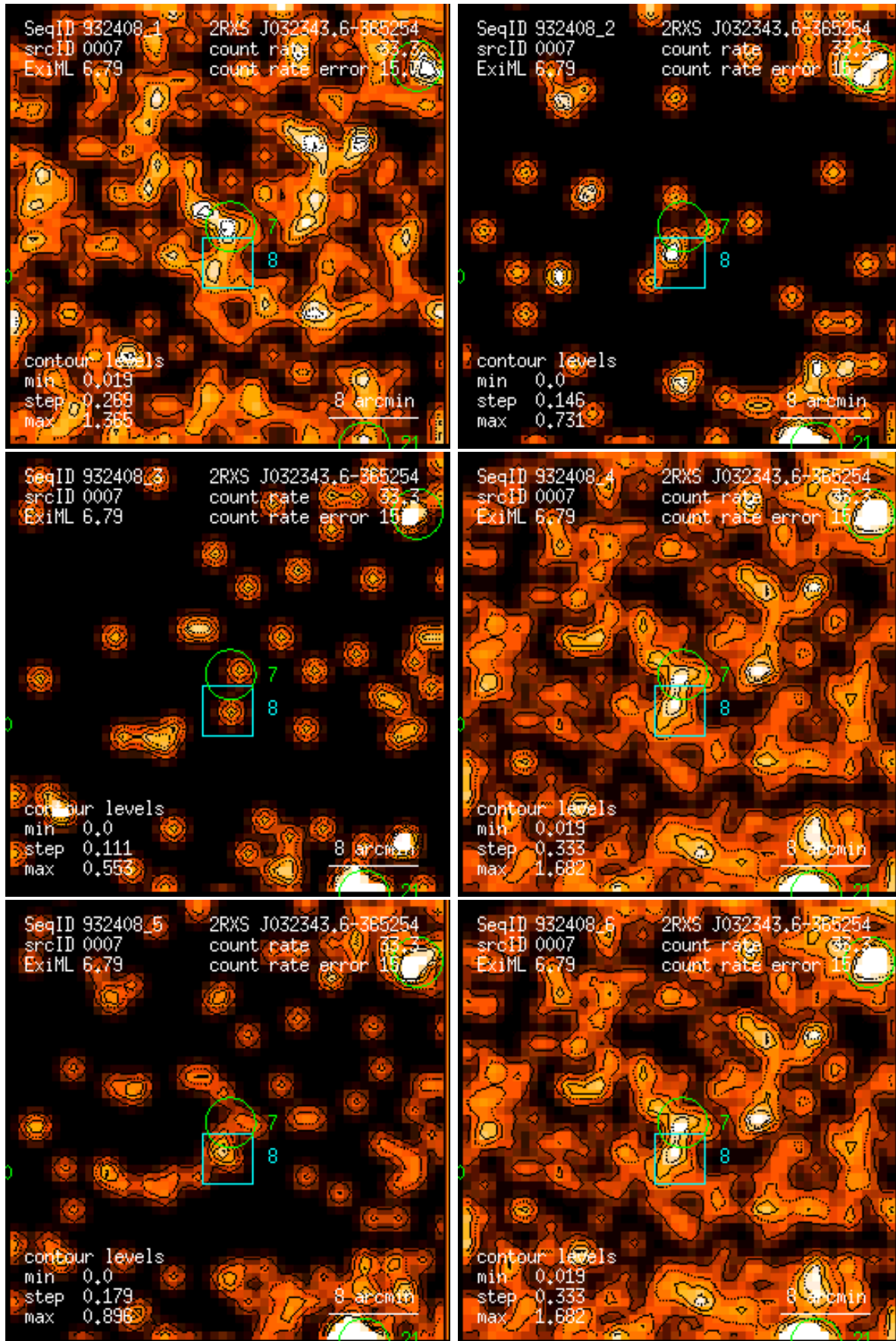
Figure 7: RASS 932408: detection 0007: band rate images, Gaussian filter: (1) PSPC channels 11 – 41, (2) 52 – 90, (3) 91 – 201, (4) 11 – 235, (5) 52 – 201, (6) 11 – 201. Broad band rates in counts/ks. Band rate contour levels in counts/ks/arcmin 2 .
