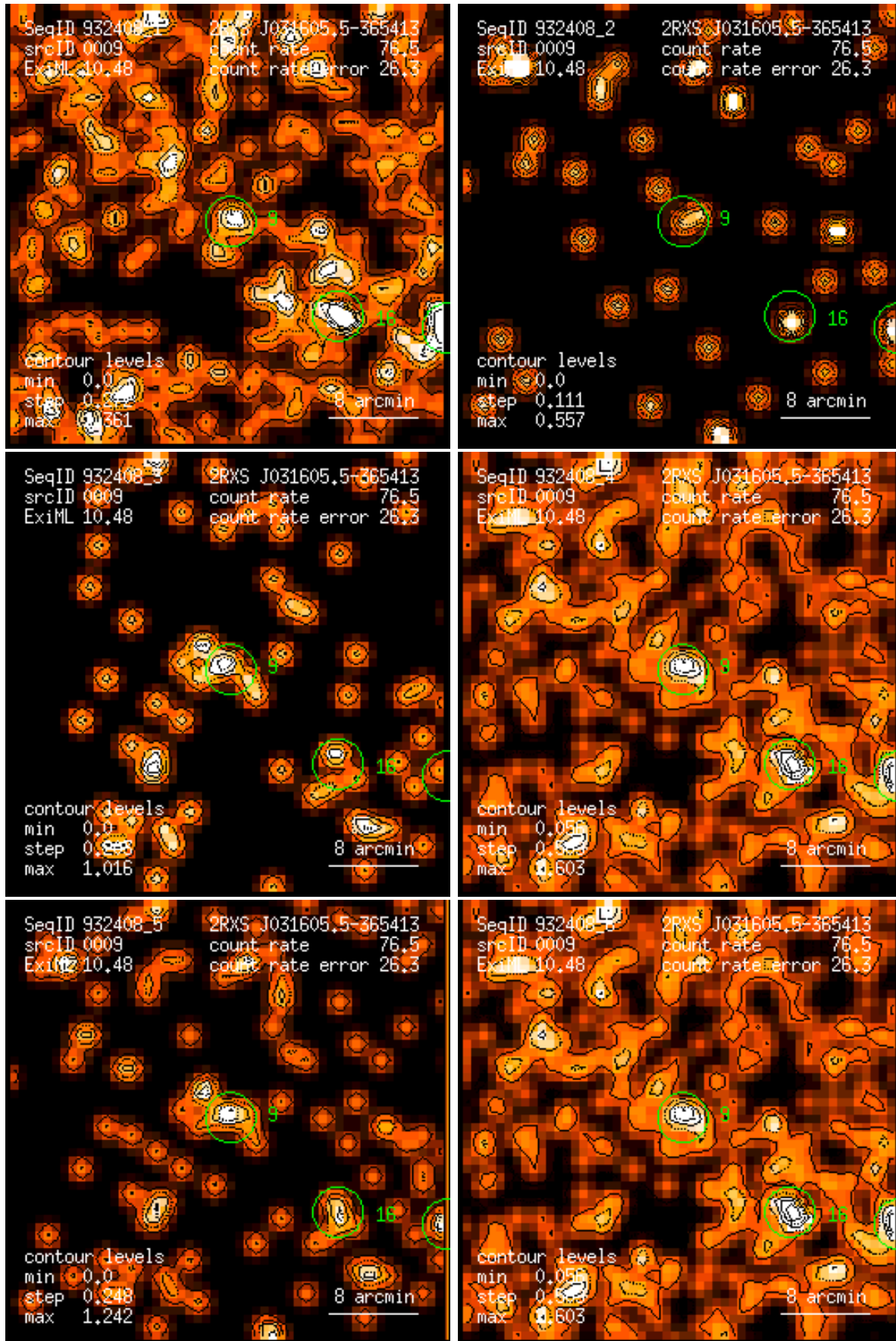
Figure 9: RASS 932408: detection 0009: band rate images, Gaussian filter: (1) PSPC channels 11 – 41, (2) 52 – 90, (3) 91 – 201, (4) 11 – 235, (5) 52 – 201, (6) 11 – 201. Broad band rates in counts/ks. Band rate contour levels in counts/ks/arcmin 2 .
