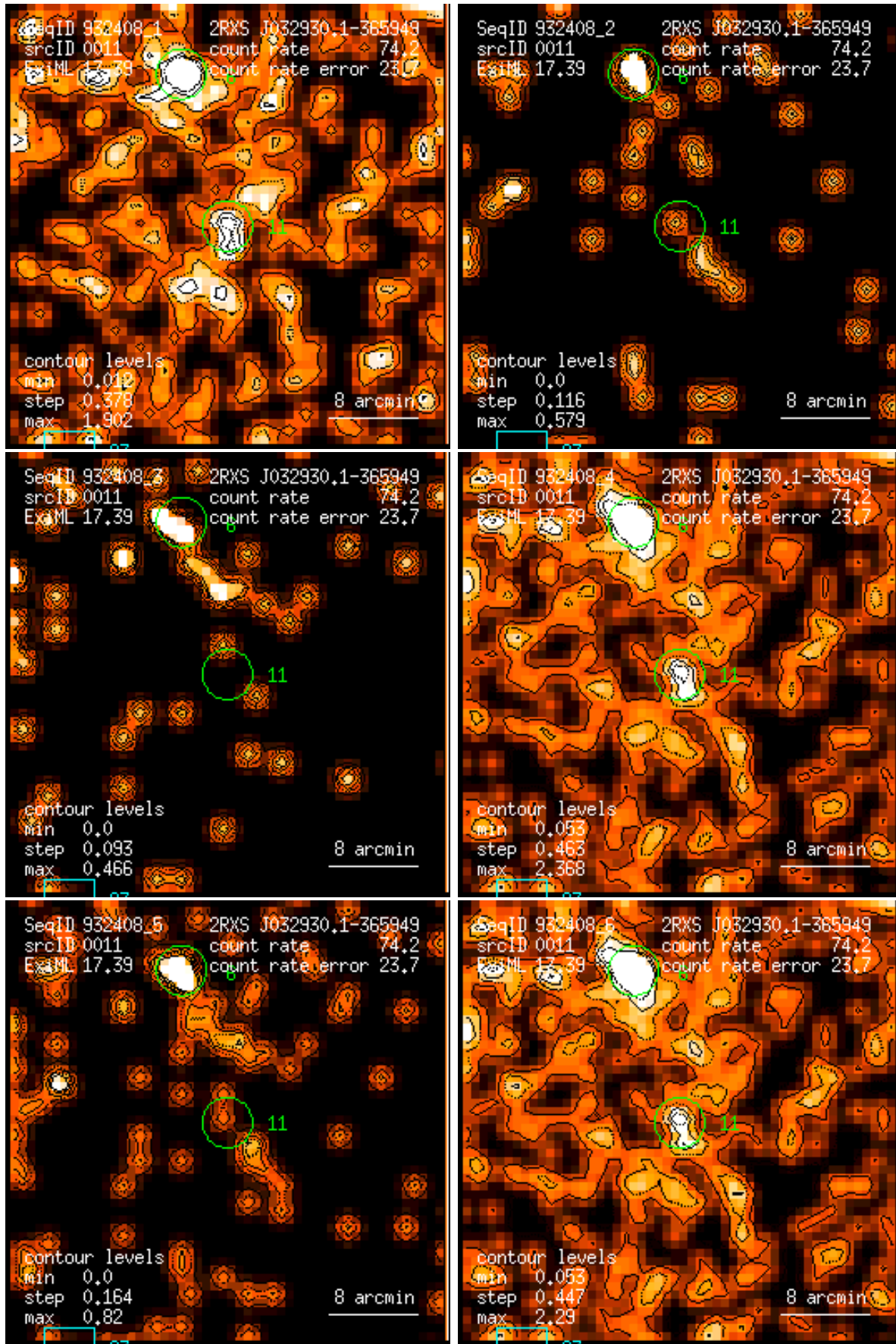
Figure 11: RASS 932408: detection 0011: band rate images, Gaussian filter: (1) PSPC channels 11 – 41, (2) 52 – 90, (3) 91 – 201, (4) 11 – 235, (5) 52 – 201, (6) 11 – 201. Broad band rates in counts/ks. Band rate contour levels in counts/ks/arcmin 2 .
