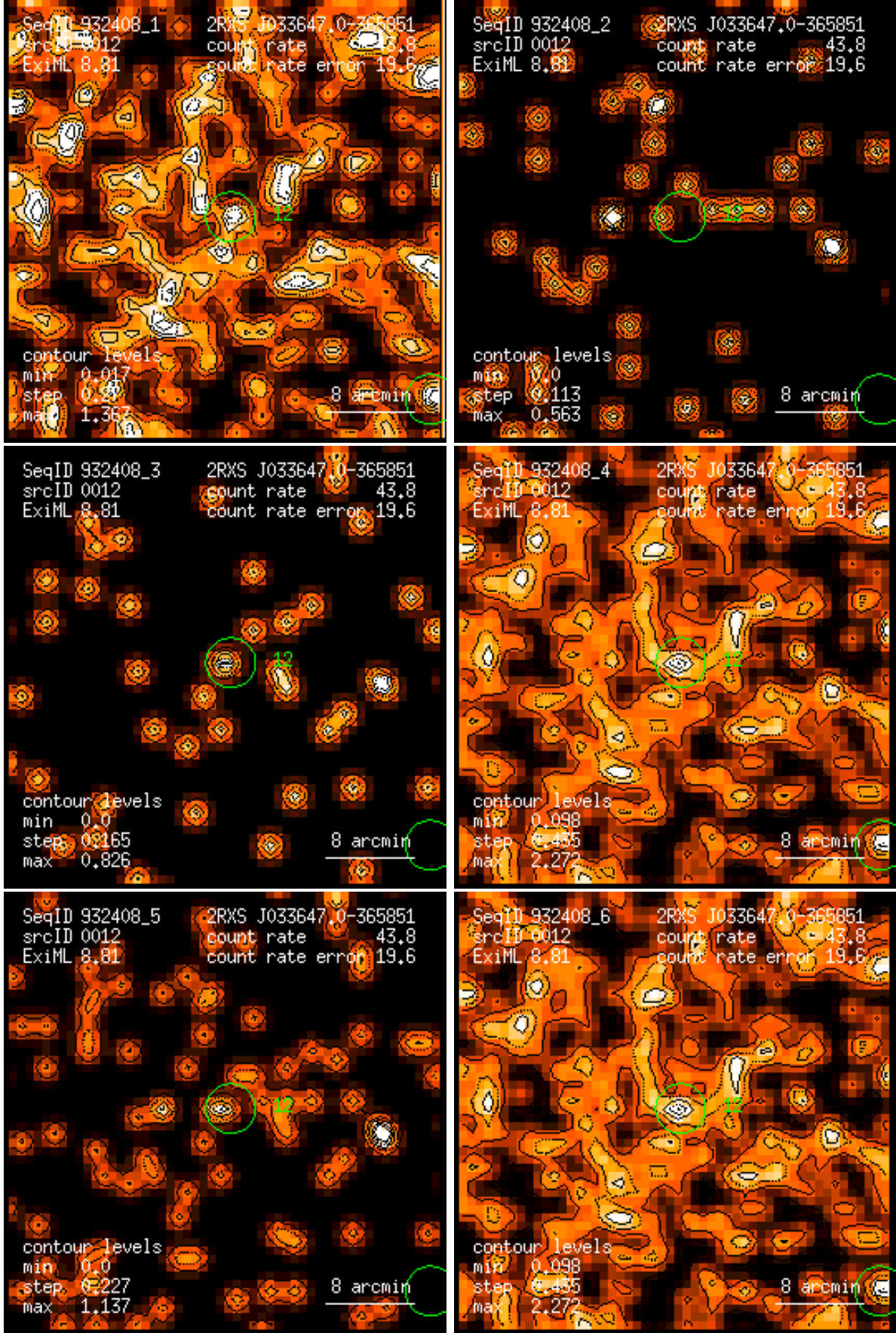
Figure 12: RASS 932408: detection 0012: band rate images, Gaussian filter: (1) PSPC channels 11 – 41, (2) 52 – 90, (3) 91 – 201, (4) 11 – 235, (5) 52 – 201, (6) 11 – 201. Broad band rates in counts/ks. Band rate contour levels in counts/ks/arcmin 2 .
