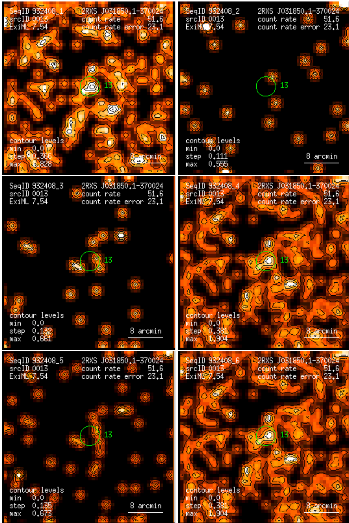
Figure 13: RASS 932408: detection 0013: band rate images, Gaussian filter: (1) PSPC channels 11 – 41, (2) 52 – 90, (3) 91 – 201, (4) 11 – 235, (5) 52 – 201, (6) 11 – 201. Broad band rates in counts/ks. Band rate contour levels in counts/ks/arcmin 2 .
