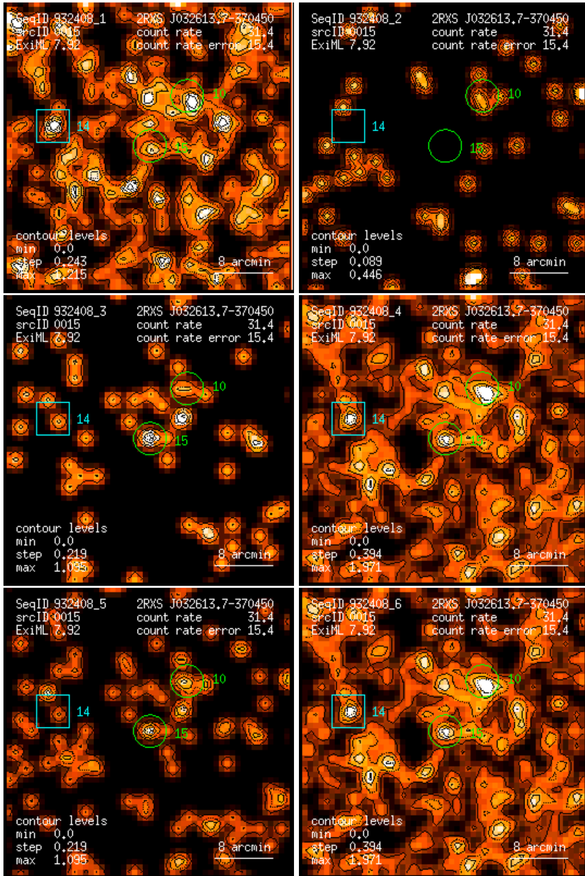
Figure 15: RASS 932408: detection 0015: band rate images, Gaussian filter: (1) PSPC channels 11 – 41, (2) 52 – 90, (3) 91 – 201, (4) 11 – 235, (5) 52 – 201, (6) 11 – 201. Broad band rates in counts/ks. Band rate contour levels in counts/ks/arcmin 2 .
