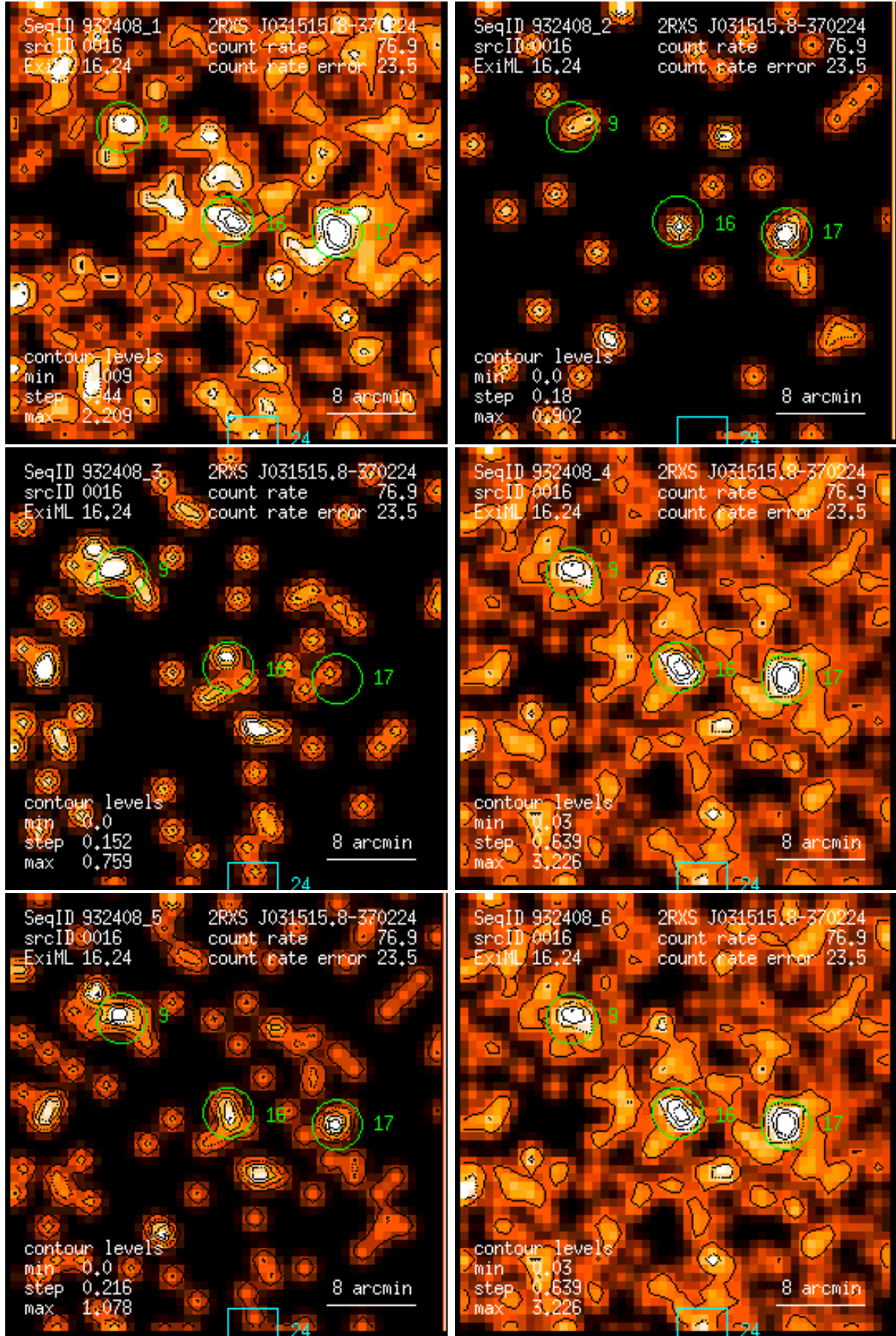
Figure 16: RASS 932408: detection 0016: band rate images, Gaussian filter: (1) PSPC channels 11 – 41, (2) 52 – 90, (3) 91 – 201, (4) 11 – 235, (5) 52 – 201, (6) 11 – 201. Broad band rates in counts/ks. Band rate contour levels in counts/ks/arcmin 2 .
