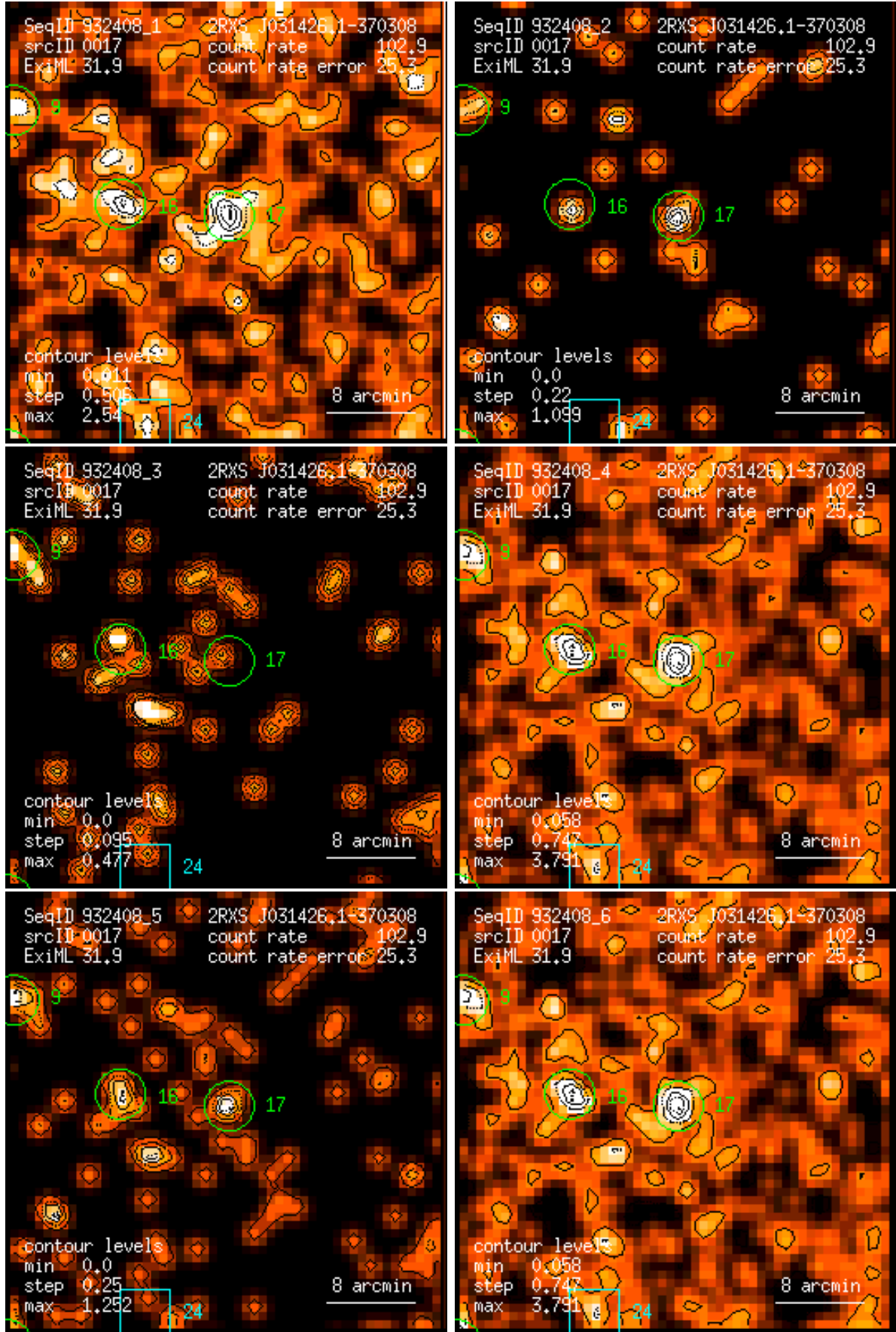
Figure 17: RASS 932408: detection 0017: band rate images, Gaussian filter: (1) PSPC channels 11 – 41, (2) 52 – 90, (3) 91 – 201, (4) 11 – 235, (5) 52 – 201, (6) 11 – 201. Broad band rates in counts/ks. Band rate contour levels in counts/ks/arcmin 2 .
