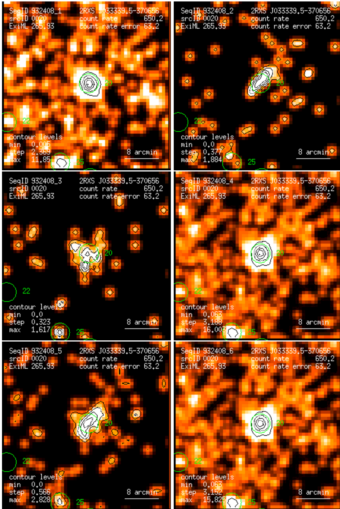
Figure 20: RASS 932408: detection 0020: band rate images, Gaussian filter: (1) PSPC channels 11 – 41, (2) 52 – 90, (3) 91 – 201, (4) 11 – 235, (5) 52 – 201, (6) 11 – 201. Broad band rates in counts/ks. Band rate contour levels in counts/ks/arcmin 2 .
