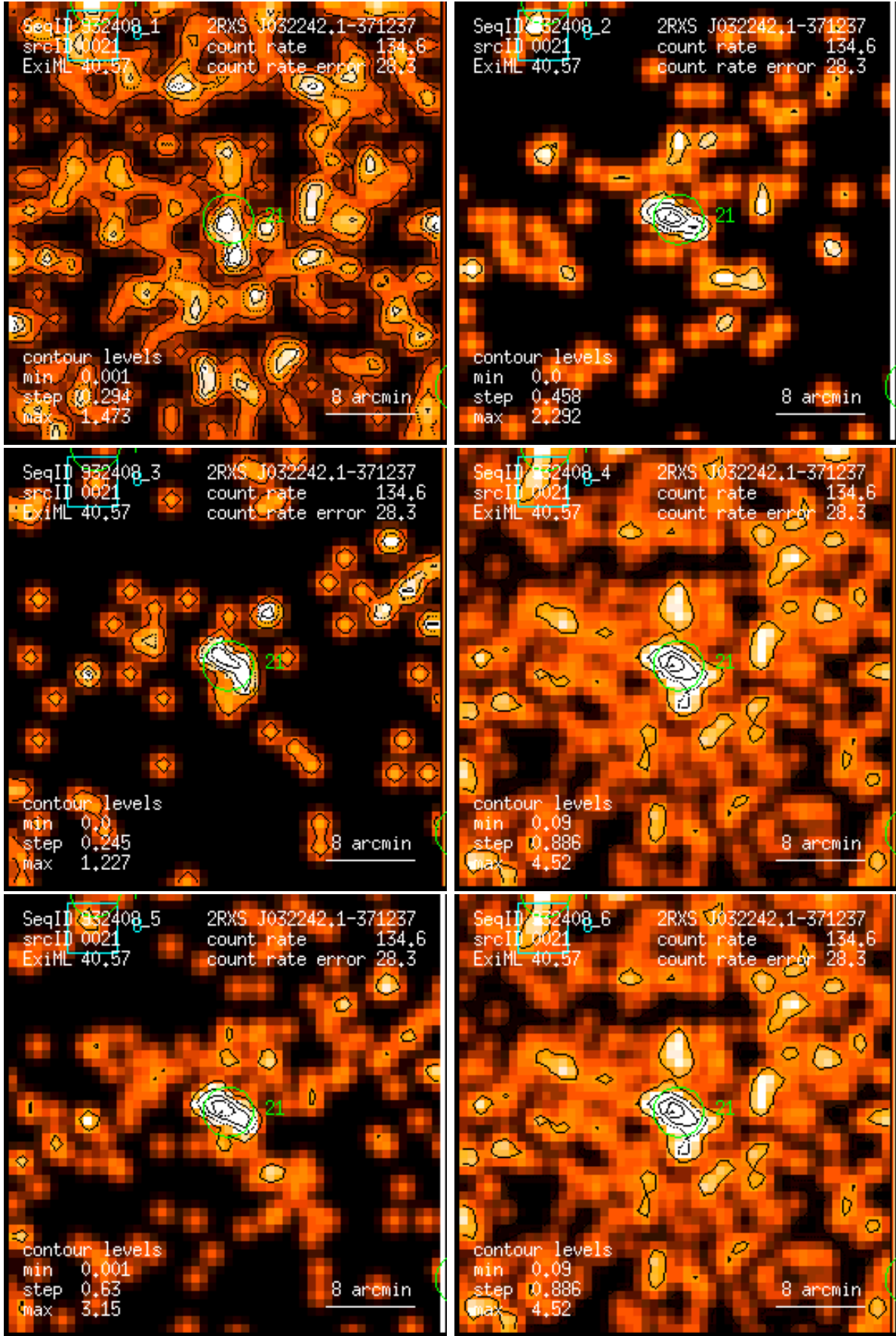
Figure 21: RASS 932408: detection 0021: band rate images, Gaussian filter: (1) PSPC channels 11 – 41, (2) 52 – 90, (3) 91 – 201, (4) 11 – 235, (5) 52 – 201, (6) 11 – 201. Broad band rates in counts/ks. Band rate contour levels in counts/ks/arcmin 2 .
