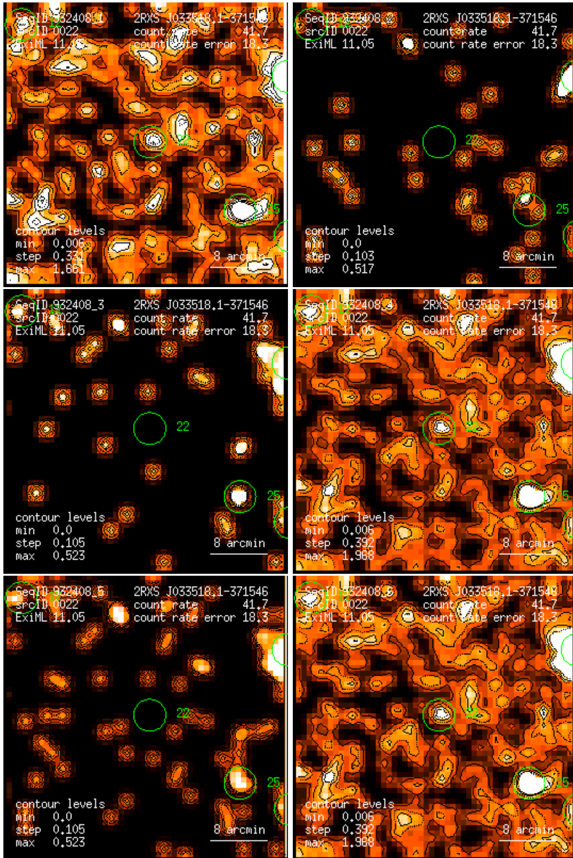
Figure 22: RASS 932408: detection 0022: band rate images, Gaussian filter: (1) PSPC channels 11 – 41, (2) 52 – 90, (3) 91 – 201, (4) 11 – 235, (5) 52 – 201, (6) 11 – 201. Broad band rates in counts/ks. Band rate contour levels in counts/ks/arcmin 2 .
