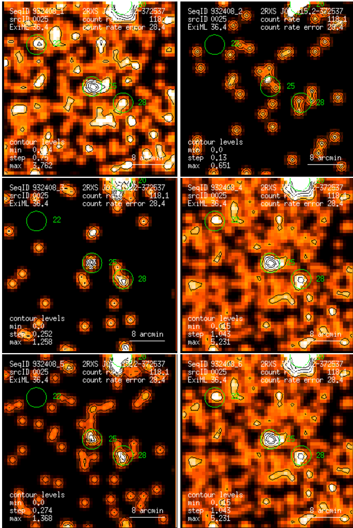
Figure 25: RASS 932408: detection 0025: band rate images, Gaussian filter: (1) PSPC channels 11 – 41, (2) 52 – 90, (3) 91 – 201, (4) 11 – 235, (5) 52 – 201, (6) 11 – 201. Broad band rates in counts/ks. Band rate contour levels in counts/ks/arcmin 2 .
