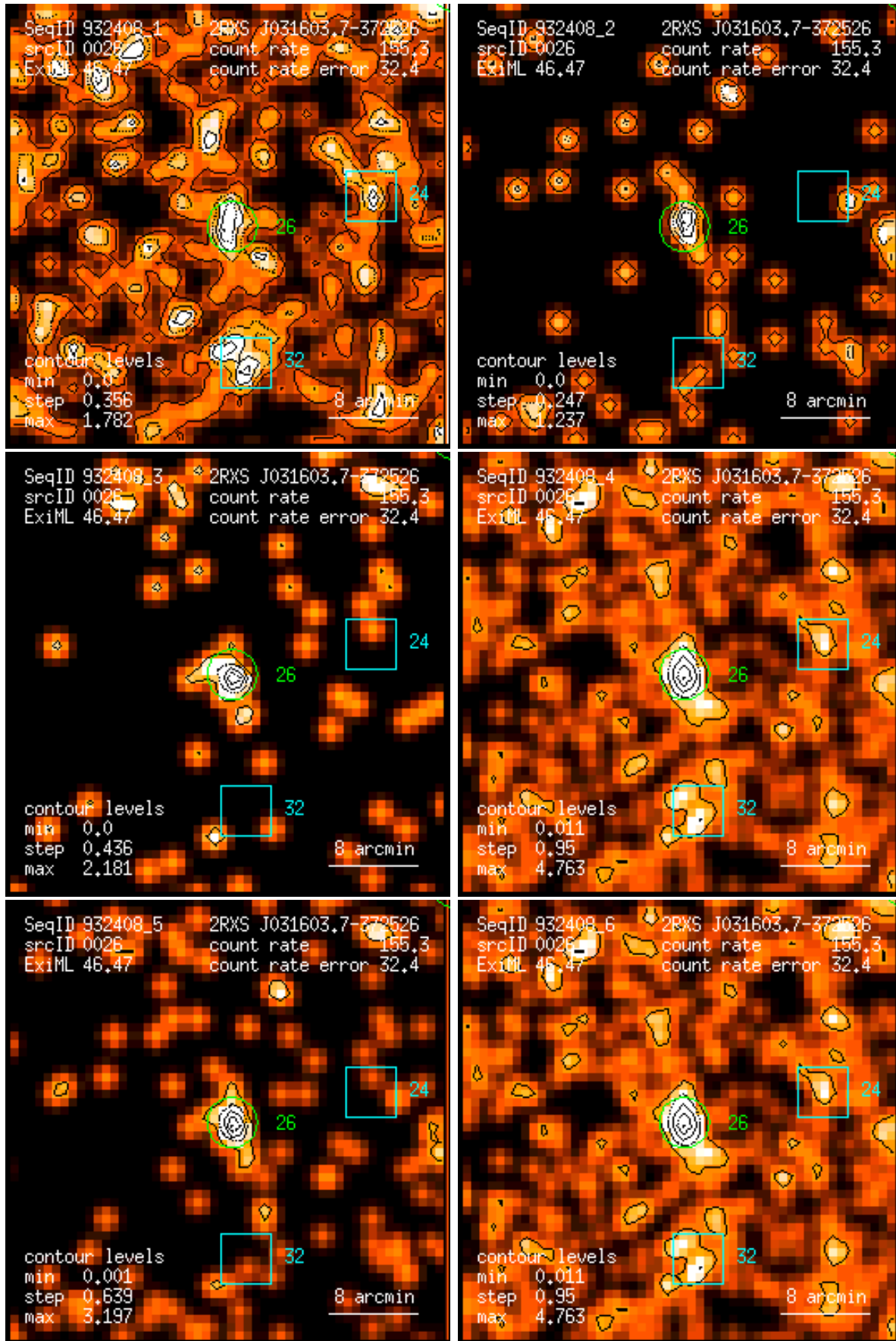
Figure 26: RASS 932408: detection 0026: band rate images, Gaussian filter: (1) PSPC channels 11 – 41, (2) 52 – 90, (3) 91 – 201, (4) 11 – 235, (5) 52 – 201, (6) 11 – 201. Broad band rates in counts/ks. Band rate contour levels in counts/ks/arcmin 2 .
