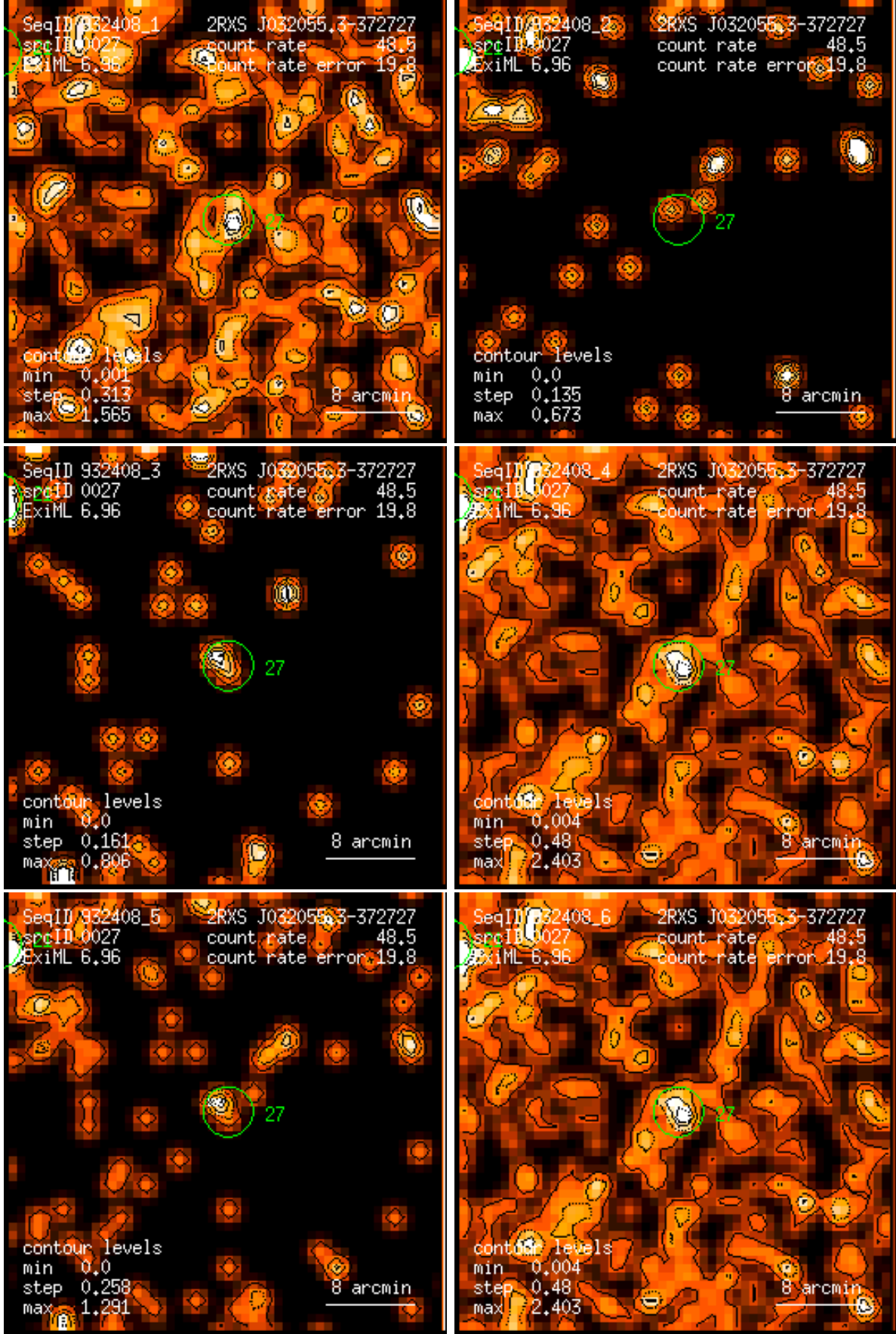
Figure 27: RASS 932408: detection 0027: band rate images, Gaussian filter: (1) PSPC channels 11 – 41, (2) 52 – 90, (3) 91 – 201, (4) 11 – 235, (5) 52 – 201, (6) 11 – 201. Broad band rates in counts/ks. Band rate contour levels in counts/ks/arcmin 2 .
