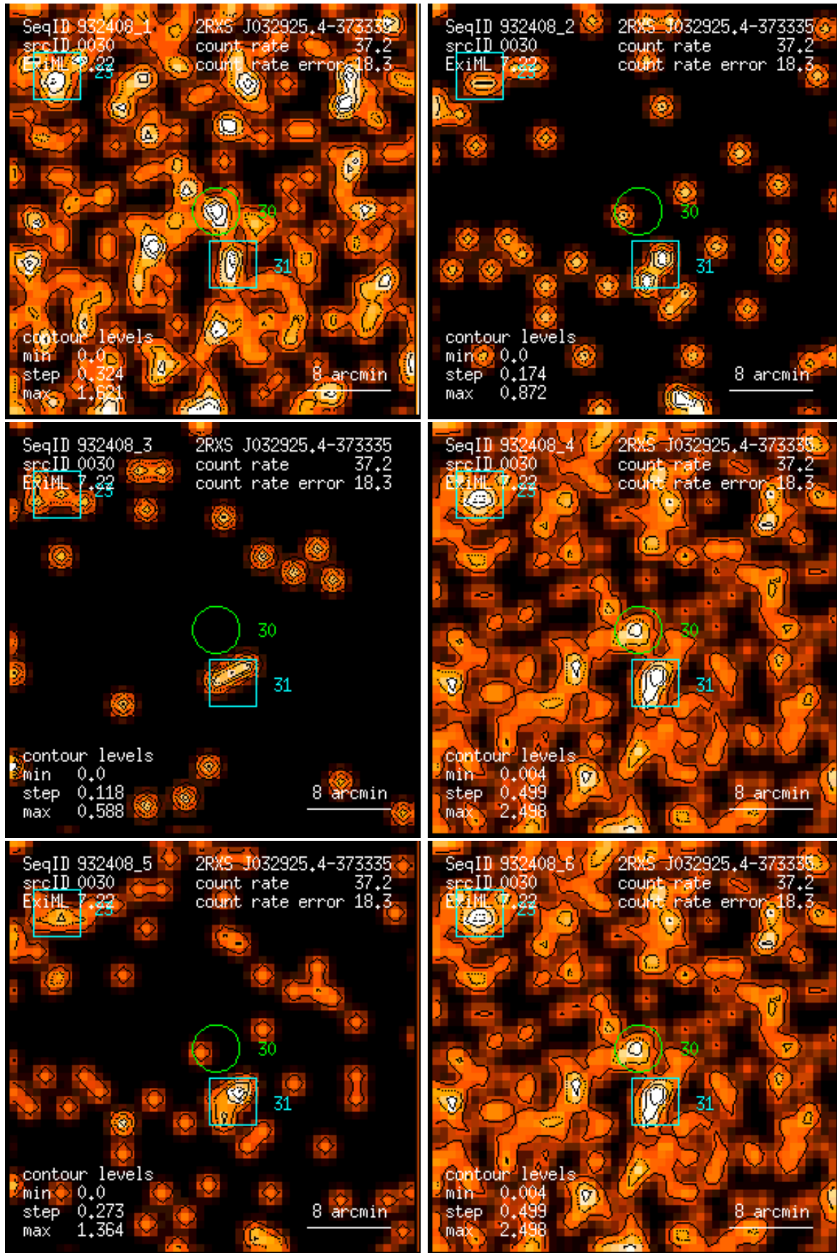
Figure 30: RASS 932408: detection 0030: band rate images, Gaussian filter: (1) PSPC channels 11 – 41, (2) 52 – 90, (3) 91 – 201, (4) 11 – 235, (5) 52 – 201, (6) 11 – 201. Broad band rates in counts/ks. Band rate contour levels in counts/ks/arcmin 2 .
