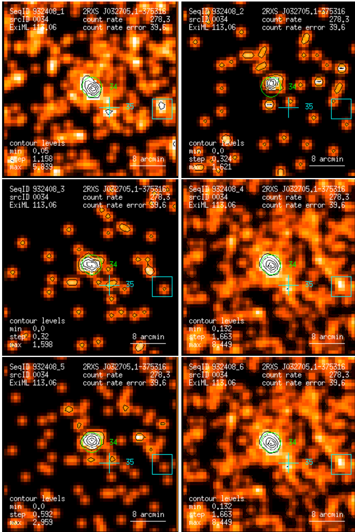
Figure 34: RASS 932408: detection 0034: band rate images, Gaussian filter: (1) PSPC channels 11 – 41, (2) 52 – 90, (3) 91 – 201, (4) 11 – 235, (5) 52 – 201, (6) 11 – 201. Broad band rates in counts/ks. Band rate contour levels in counts/ks/arcmin 2 .
