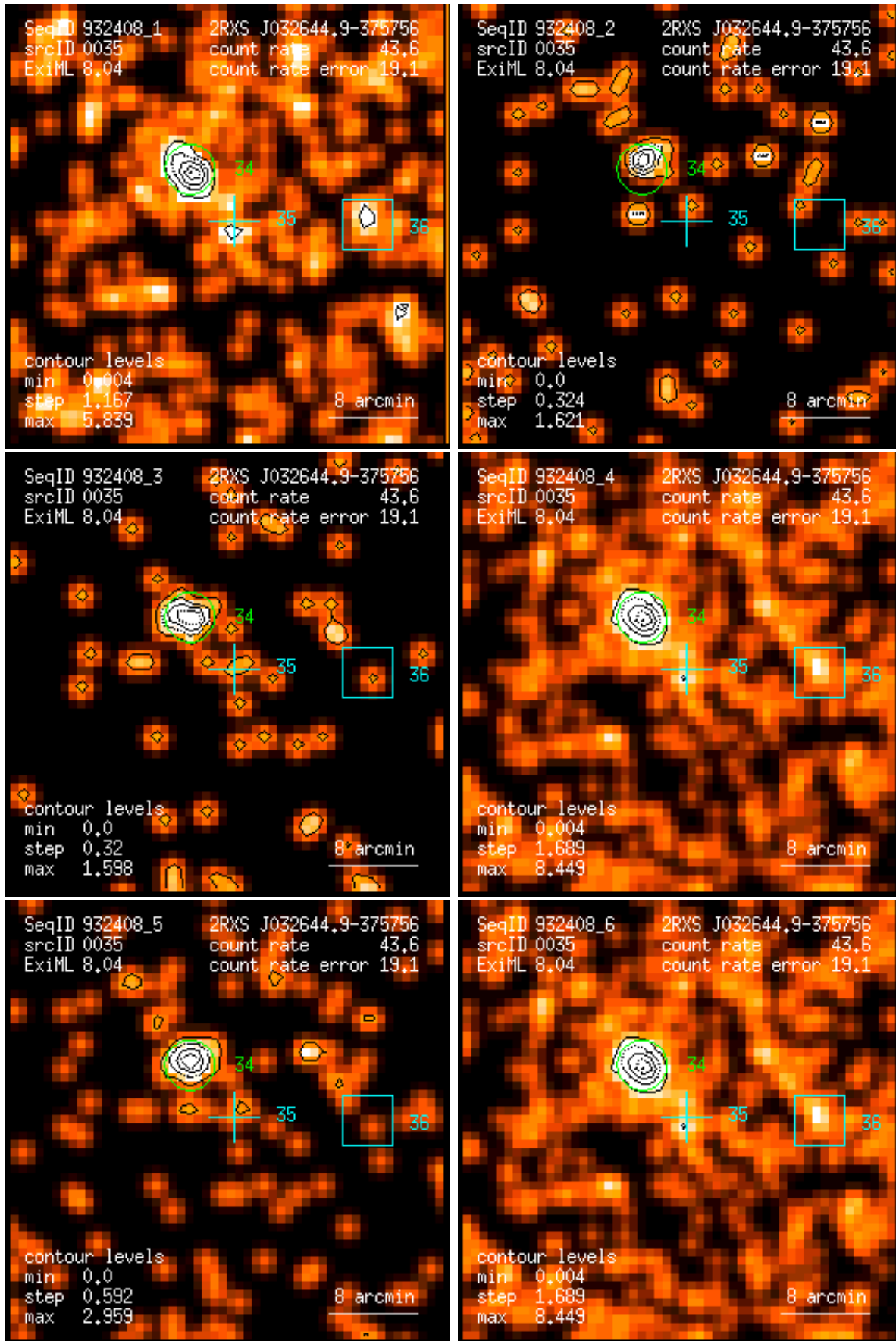
Figure 35: RASS 932408: detection 0035: band rate images, Gaussian filter: (1) PSPC channels 11 – 41, (2) 52 – 90, (3) 91 – 201, (4) 11 – 235, (5) 52 – 201, (6) 11 – 201. Broad band rates in counts/ks. Band rate contour levels in counts/ks/arcmin 2 .
