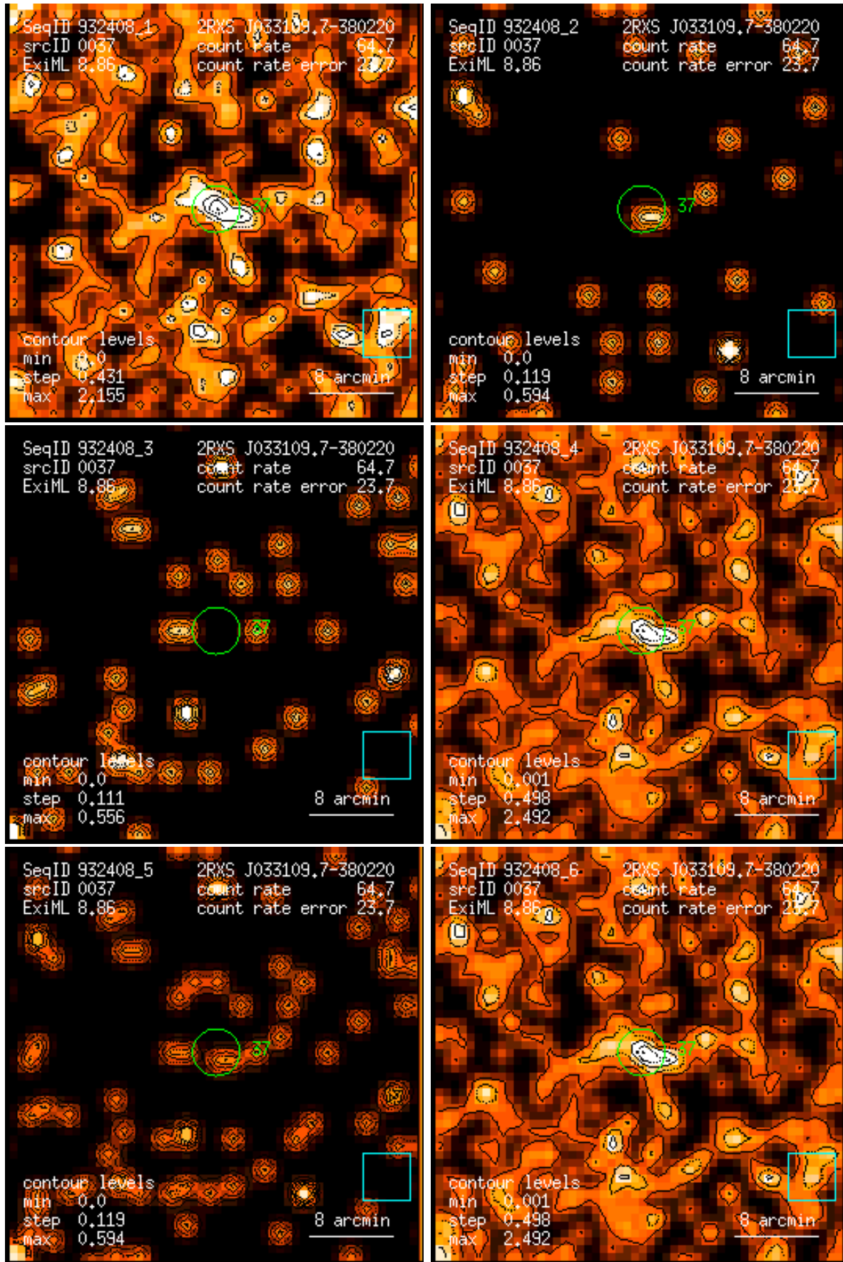
Figure 37: RASS 932408: detection 0037: band rate images, Gaussian filter: (1) PSPC channels 11 – 41, (2) 52 – 90, (3) 91 – 201, (4) 11 – 235, (5) 52 – 201, (6) 11 – 201. Broad band rates in counts/ks. Band rate contour levels in counts/ks/arcmin 2 .
