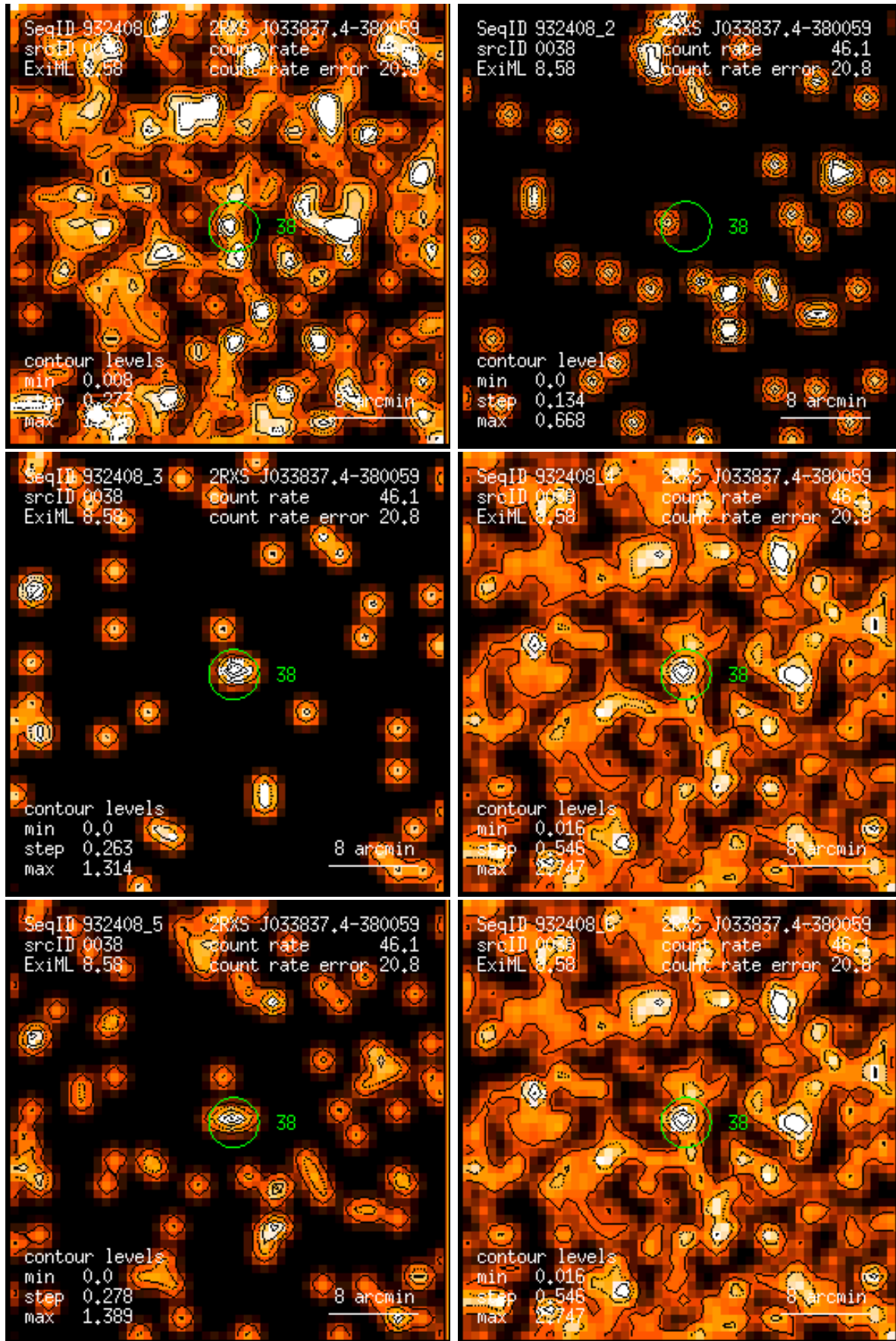
Figure 38: RASS 932408: detection 0038: band rate images, Gaussian filter: (1) PSPC channels 11 – 41, (2) 52 – 90, (3) 91 – 201, (4) 11 – 235, (5) 52 – 201, (6) 11 – 201. Broad band rates in counts/ks. Band rate contour levels in counts/ks/arcmin 2 .
