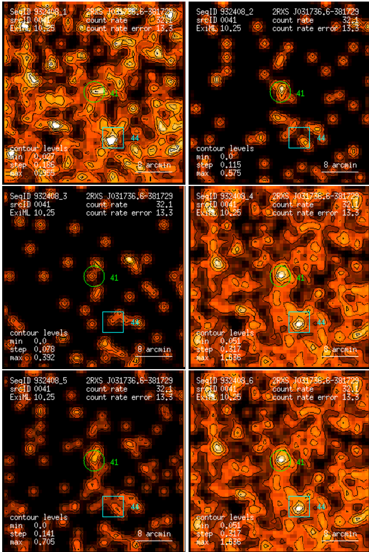
Figure 41: RASS 932408: detection 0041: band rate images, Gaussian filter: (1) PSPC channels 11 – 41, (2) 52 – 90, (3) 91 – 201, (4) 11 – 235, (5) 52 – 201, (6) 11 – 201. Broad band rates in counts/ks. Band rate contour levels in counts/ks/arcmin 2 .
