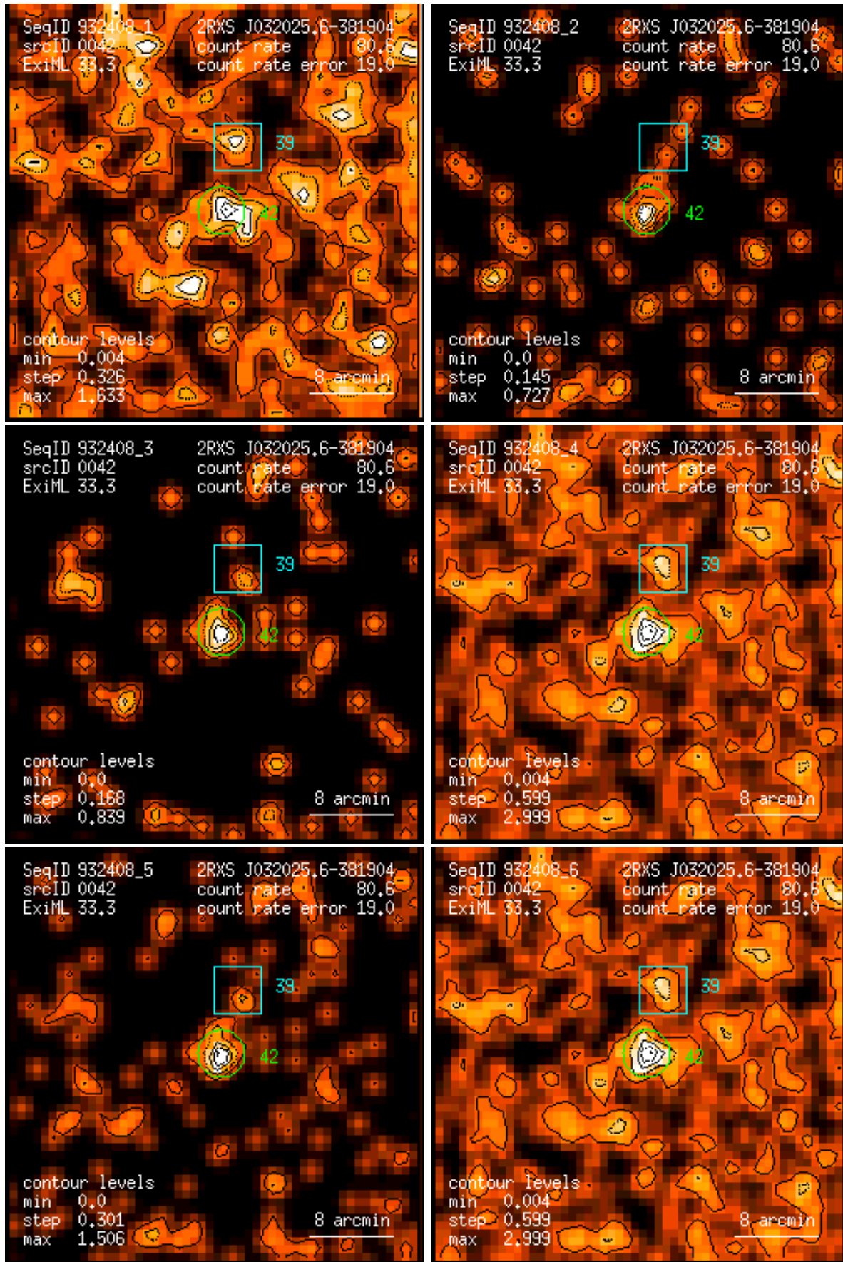
Figure 42: RASS 932408: detection 0042: band rate images, Gaussian filter: (1) PSPC channels 11 – 41, (2) 52 – 90, (3) 91 – 201, (4) 11 – 235, (5) 52 – 201, (6) 11 – 201. Broad band rates in counts/ks. Band rate contour levels in counts/ks/arcmin 2 .
