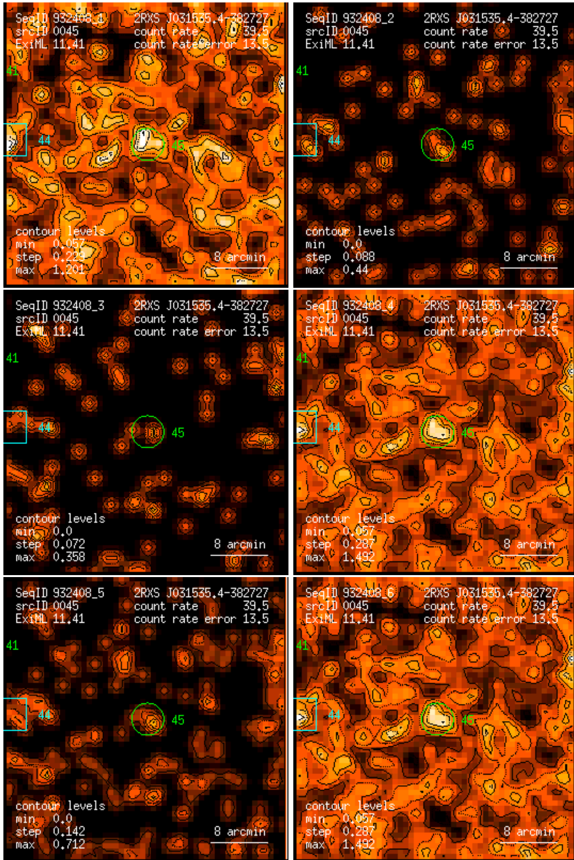
Figure 45: RASS 932408: detection 0045: band rate images, Gaussian filter: (1) PSPC channels 11 – 41, (2) 52 – 90, (3) 91 – 201, (4) 11 – 235, (5) 52 – 201, (6) 11 – 201. Broad band rates in counts/ks. Band rate contour levels in counts/ks/arcmin 2 .
