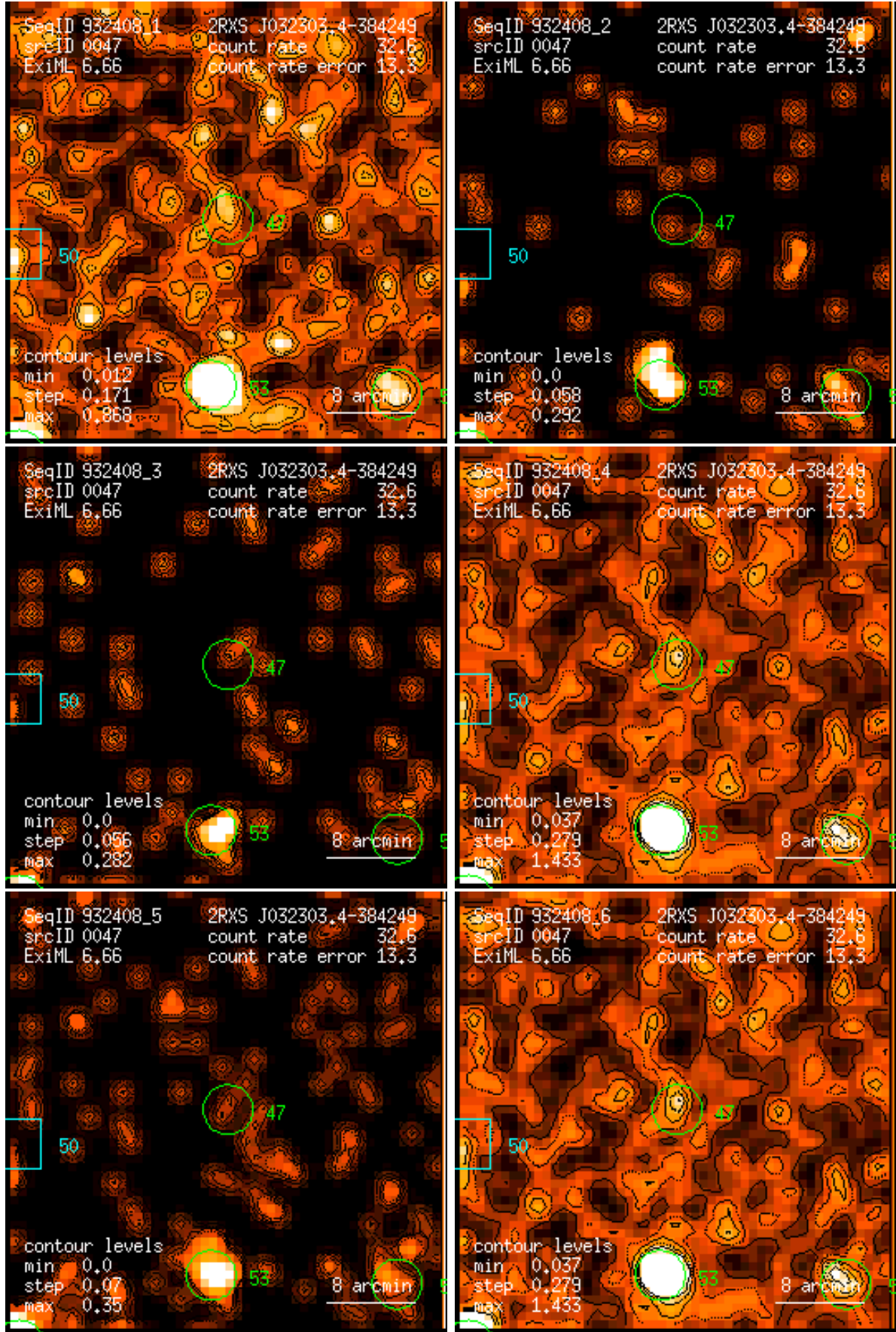
Figure 47: RASS 932408: detection 0047: band rate images, Gaussian filter: (1) PSPC channels 11 – 41, (2) 52 – 90, (3) 91 – 201, (4) 11 – 235, (5) 52 – 201, (6) 11 – 201. Broad band rates in counts/ks. Band rate contour levels in counts/ks/arcmin 2 .
