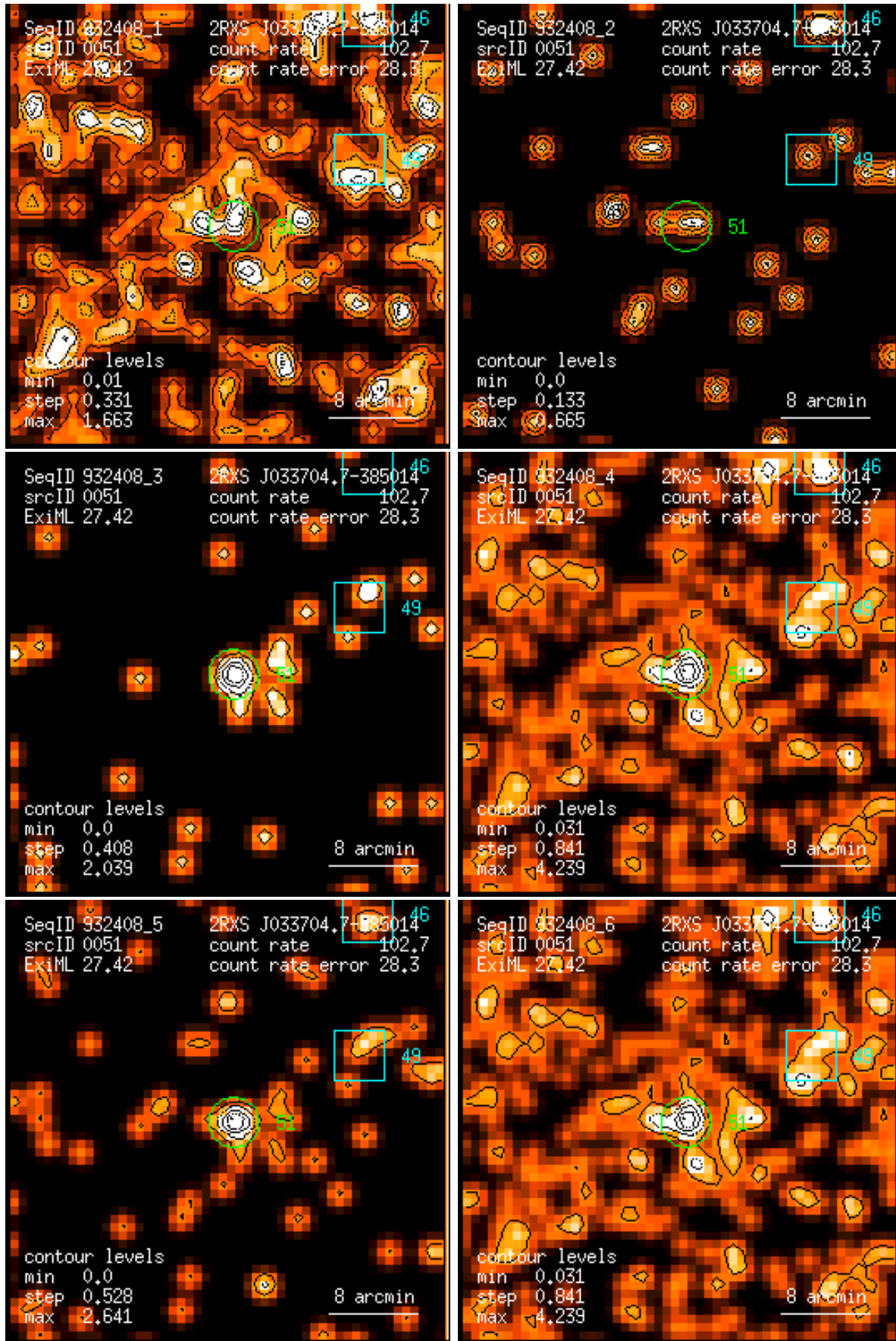
Figure 51: RASS 932408: detection 0051: band rate images, Gaussian filter: (1) PSPC channels 11 – 41, (2) 52 – 90, (3) 91 – 201, (4) 11 – 235, (5) 52 – 201, (6) 11 – 201. Broad band rates in counts/ks. Band rate contour levels in counts/ks/arcmin 2 .
