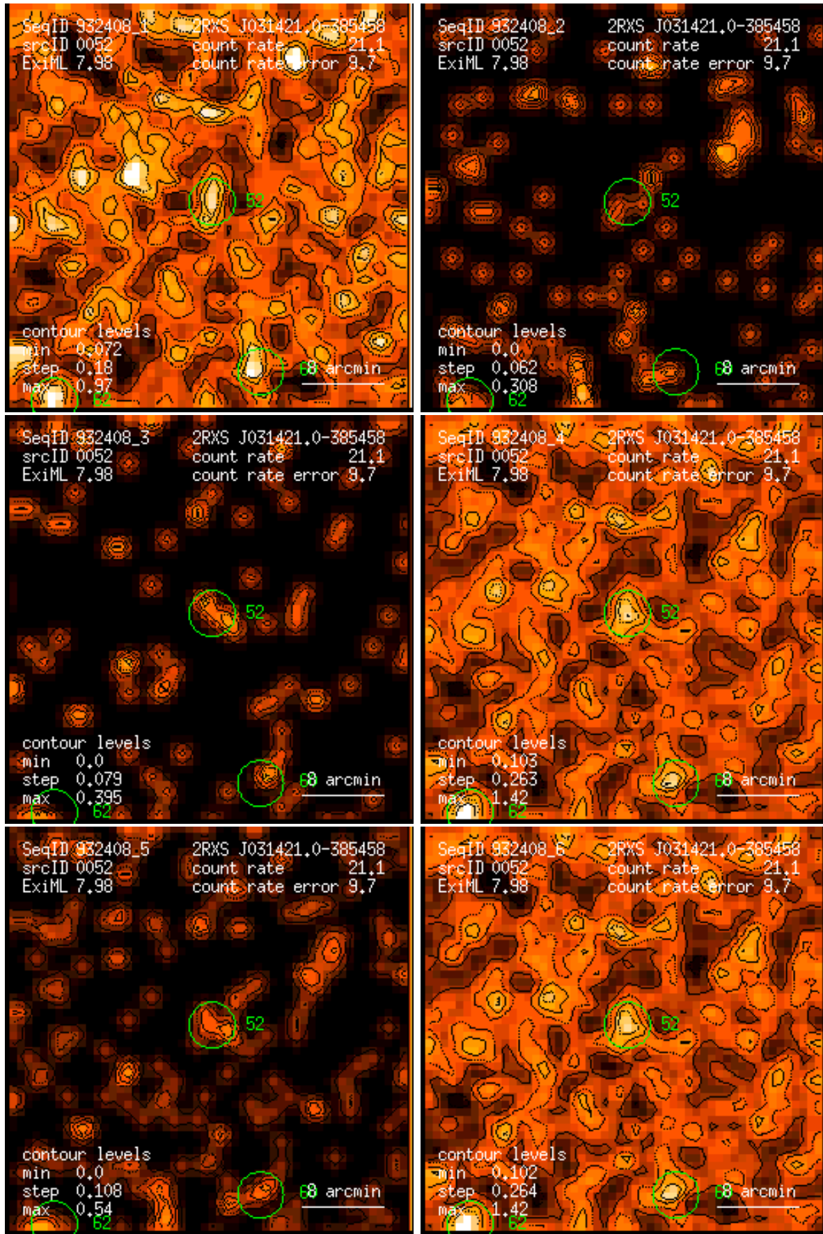
Figure 52: RASS 932408: detection 0052: band rate images, Gaussian filter: (1) PSPC channels 11 – 41, (2) 52 – 90, (3) 91 – 201, (4) 11 – 235, (5) 52 – 201, (6) 11 – 201. Broad band rates in counts/ks. Band rate contour levels in counts/ks/arcmin 2 .
