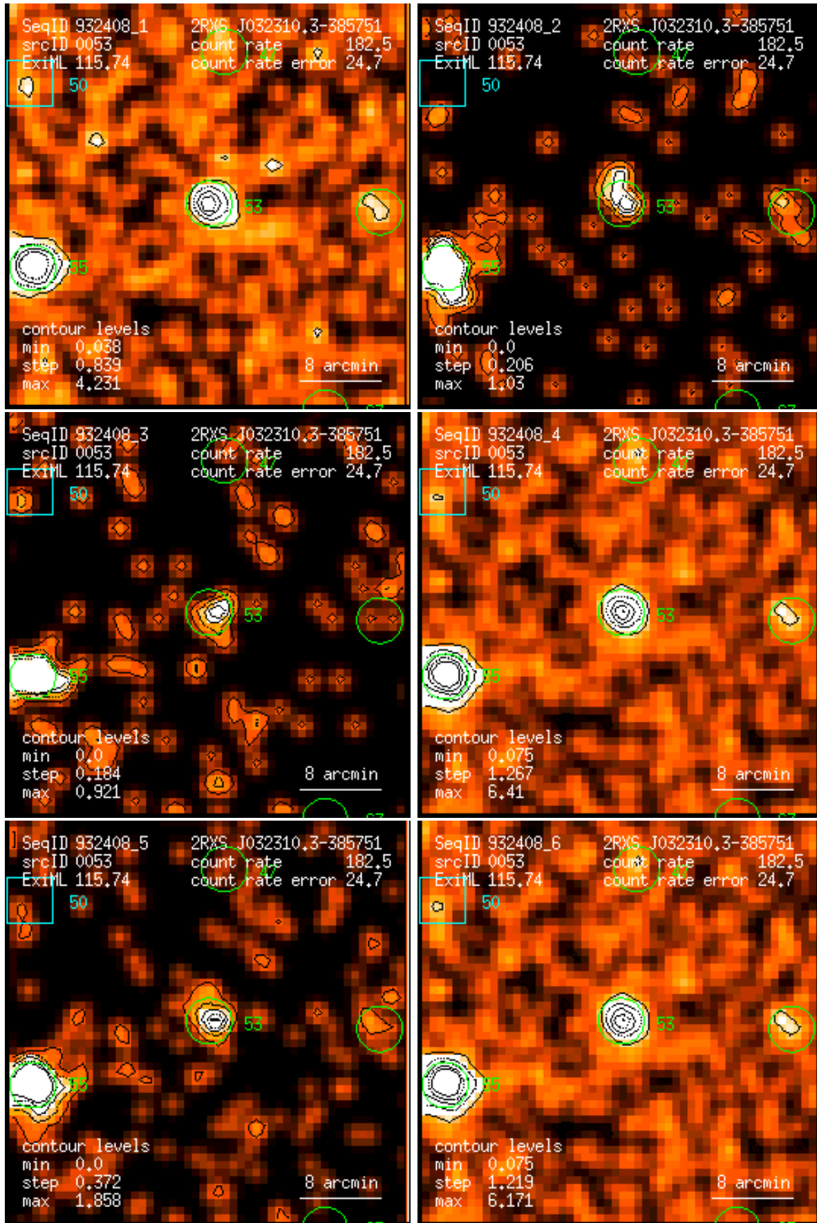
Figure 53: RASS 932408: detection 0053: band rate images, Gaussian filter: (1) PSPC channels 11 – 41, (2) 52 – 90, (3) 91 – 201, (4) 11 – 235, (5) 52 – 201, (6) 11 – 201. Broad band rates in counts/ks. Band rate contour levels in counts/ks/arcmin 2 .
