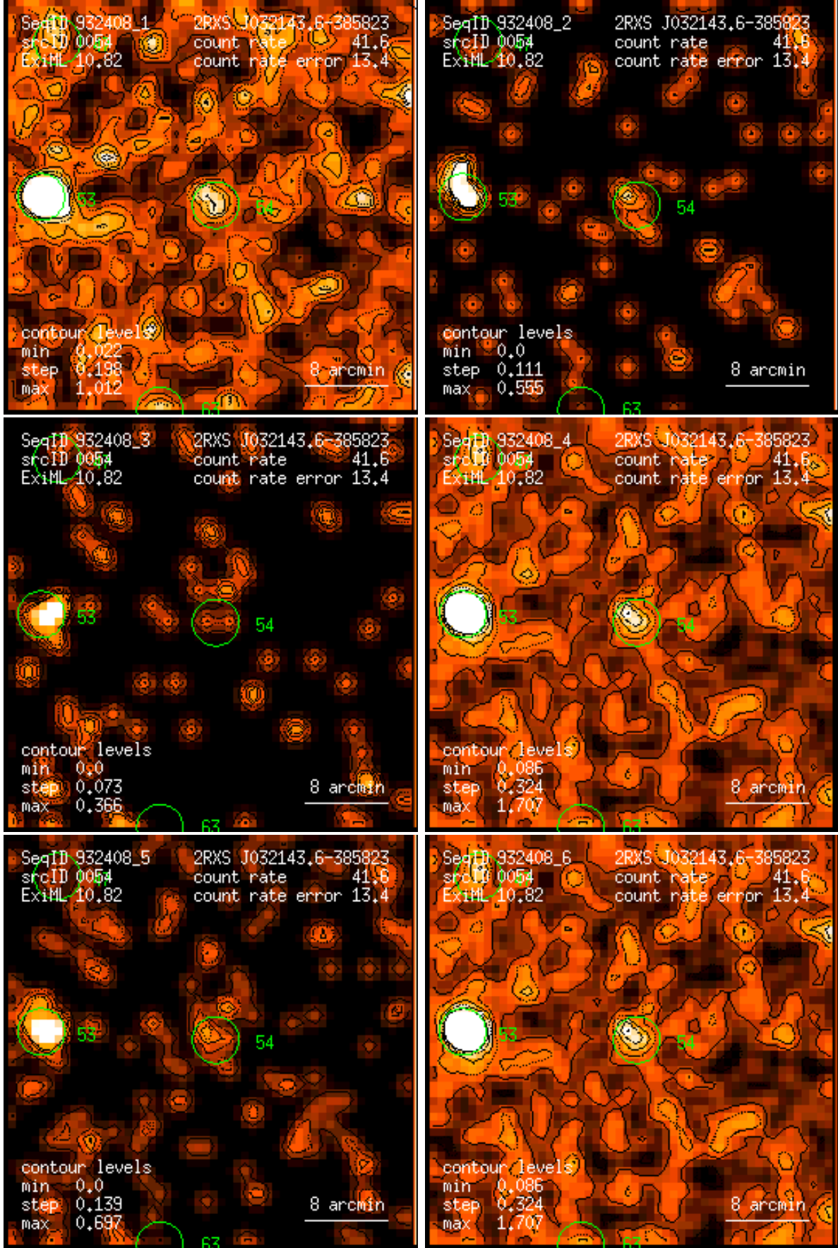
Figure 54: RASS 932408: detection 0054: band rate images, Gaussian filter: (1) PSPC channels 11 – 41, (2) 52 – 90, (3) 91 – 201, (4) 11 – 235, (5) 52 – 201, (6) 11 – 201. Broad band rates in counts/ks. Band rate contour levels in counts/ks/arcmin 2 .
