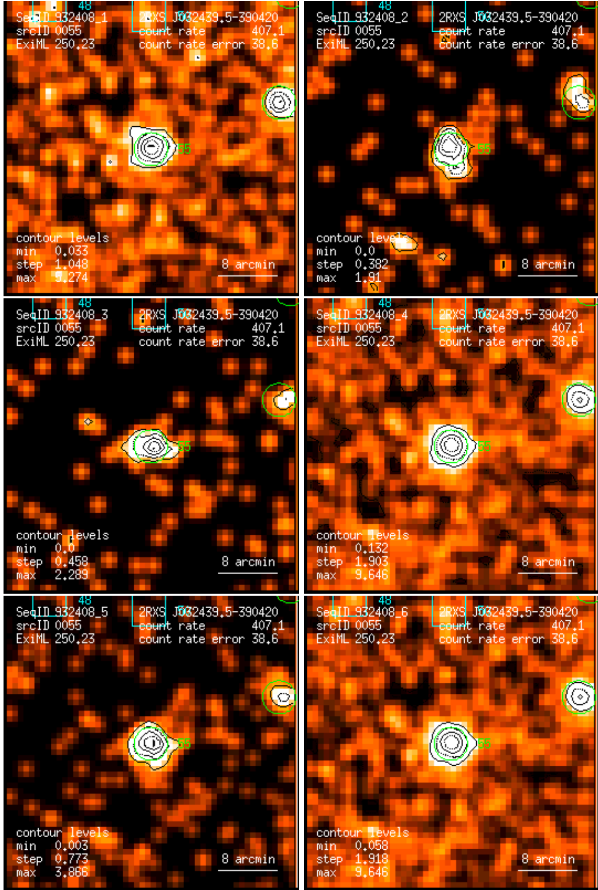
Figure 55: RASS 932408: detection 0055: band rate images, Gaussian filter: (1) PSPC channels 11 – 41, (2) 52 – 90, (3) 91 – 201, (4) 11 – 235, (5) 52 – 201, (6) 11 – 201. Broad band rates in counts/ks. Band rate contour levels in counts/ks/arcmin 2 .
