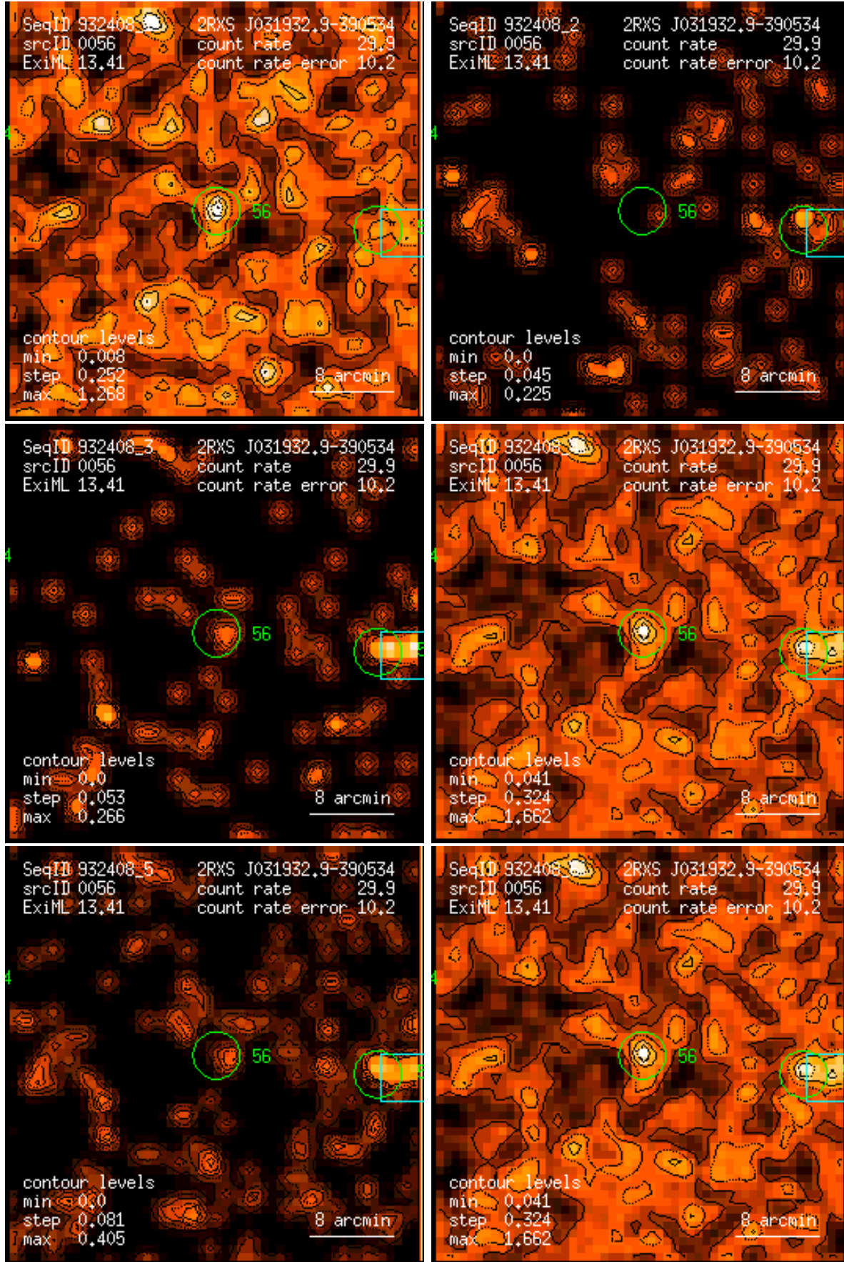
Figure 56: RASS 932408: detection 0056: band rate images, Gaussian filter: (1) PSPC channels 11 – 41, (2) 52 – 90, (3) 91 – 201, (4) 11 – 235, (5) 52 – 201, (6) 11 – 201. Broad band rates in counts/ks. Band rate contour levels in counts/ks/arcmin 2 .
