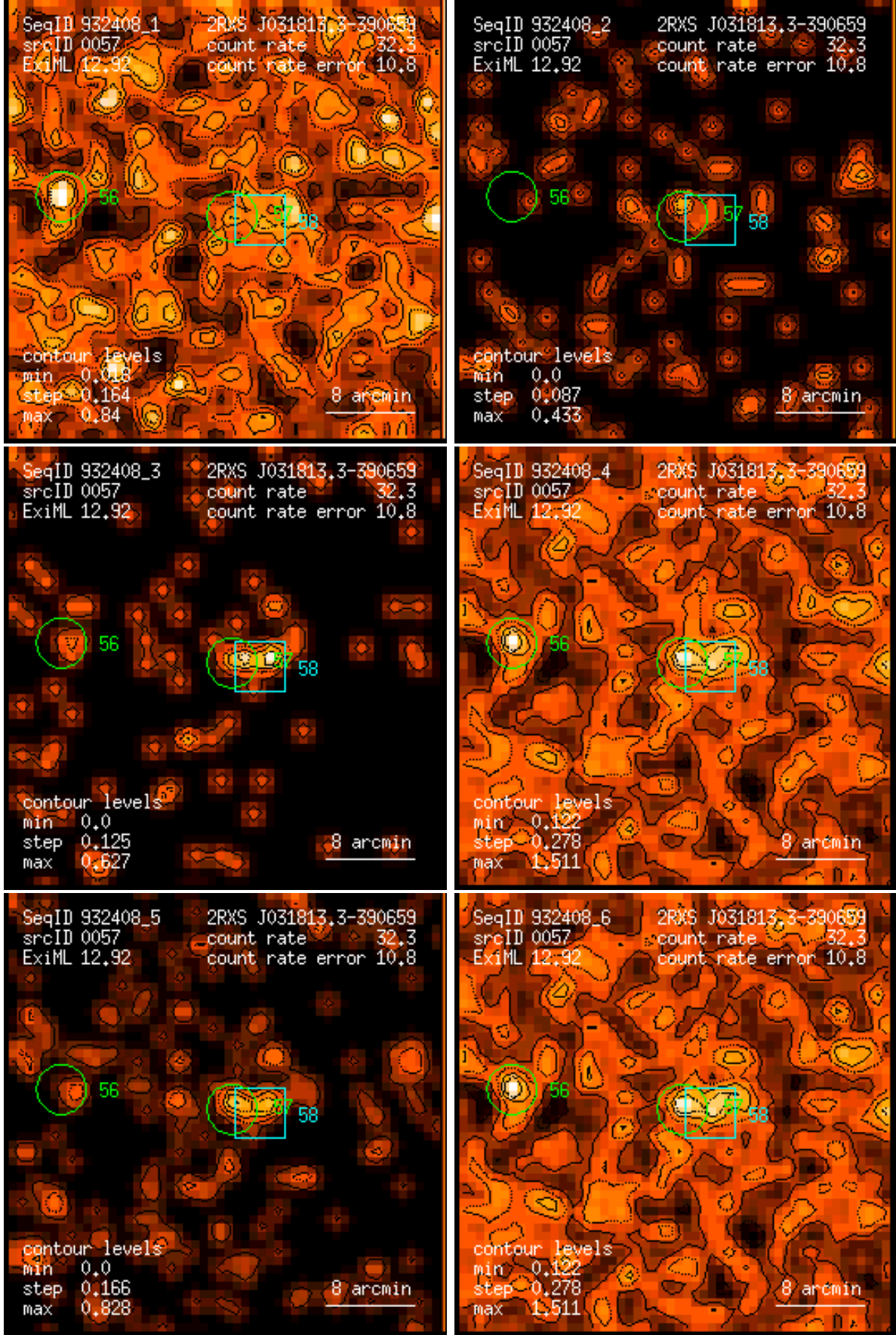
Figure 57: RASS 932408: detection 0057: band rate images, Gaussian filter: (1) PSPC channels 11 – 41, (2) 52 – 90, (3) 91 – 201, (4) 11 – 235, (5) 52 – 201, (6) 11 – 201. Broad band rates in counts/ks. Band rate contour levels in counts/ks/arcmin 2 .
