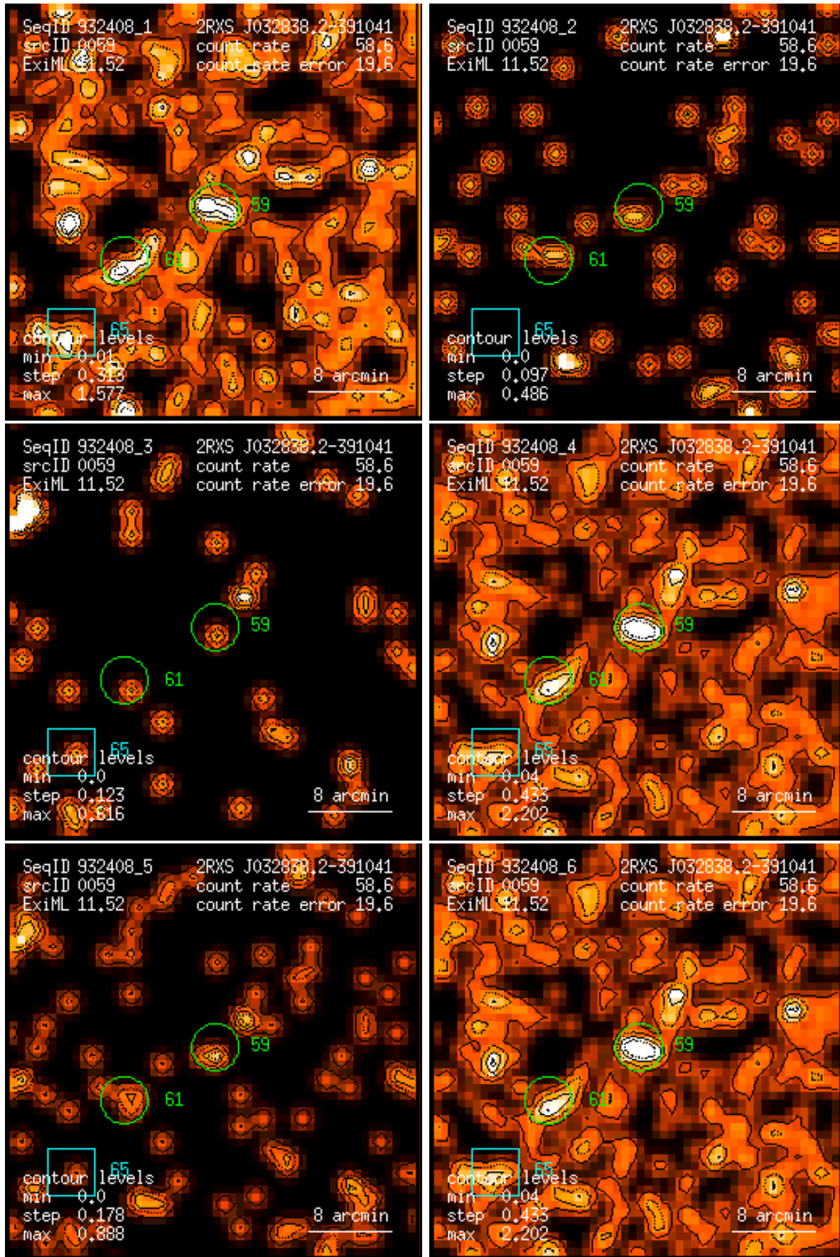
Figure 59: RASS 932408: detection 0059: band rate images, Gaussian filter: (1) PSPC channels 11 – 41, (2) 52 – 90, (3) 91 – 201, (4) 11 – 235, (5) 52 – 201, (6) 11 – 201. Broad band rates in counts/ks. Band rate contour levels in counts/ks/arcmin 2 .
