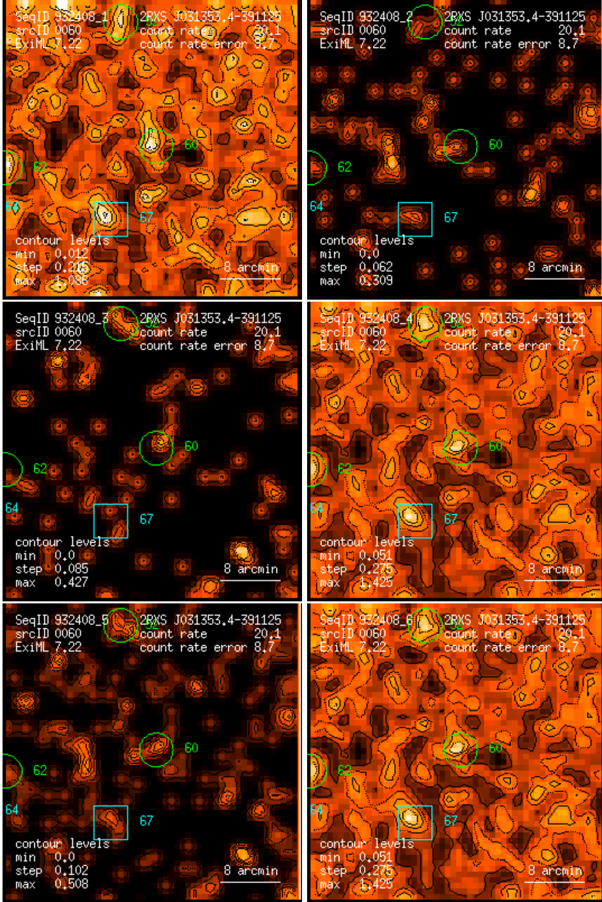
Figure 60: RASS 932408: detection 0060: band rate images, Gaussian filter: (1) PSPC channels 11 – 41, (2) 52 – 90, (3) 91 – 201, (4) 11 – 235, (5) 52 – 201, (6) 11 – 201. Broad band rates in counts/ks. Band rate contour levels in counts/ks/arcmin 2 .
