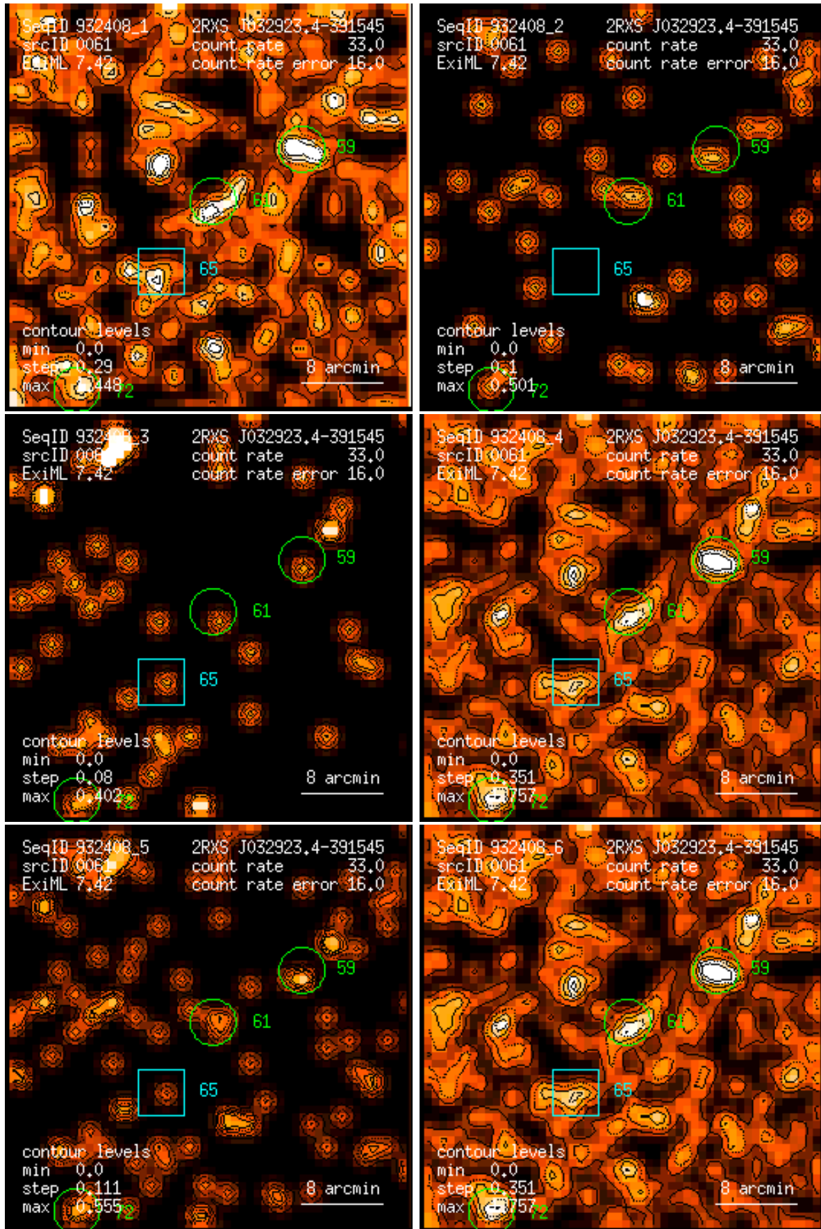
Figure 61: RASS 932408: detection 0061: band rate images, Gaussian filter: (1) PSPC channels 11 – 41, (2) 52 – 90, (3) 91 – 201, (4) 11 – 235, (5) 52 – 201, (6) 11 – 201. Broad band rates in counts/ks. Band rate contour levels in counts/ks/arcmin 2 .
