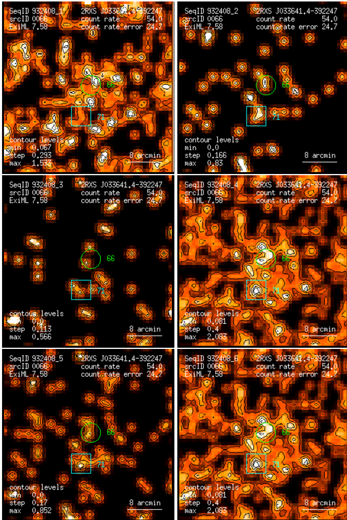
Figure 66: RASS 932408: detection 0066: band rate images, Gaussian filter: (1) PSPC channels 11 – 41, (2) 52 – 90, (3) 91 – 201, (4) 11 – 235, (5) 52 – 201, (6) 11 – 201. Broad band rates in counts/ks. Band rate contour levels in counts/ks/arcmin 2 .
