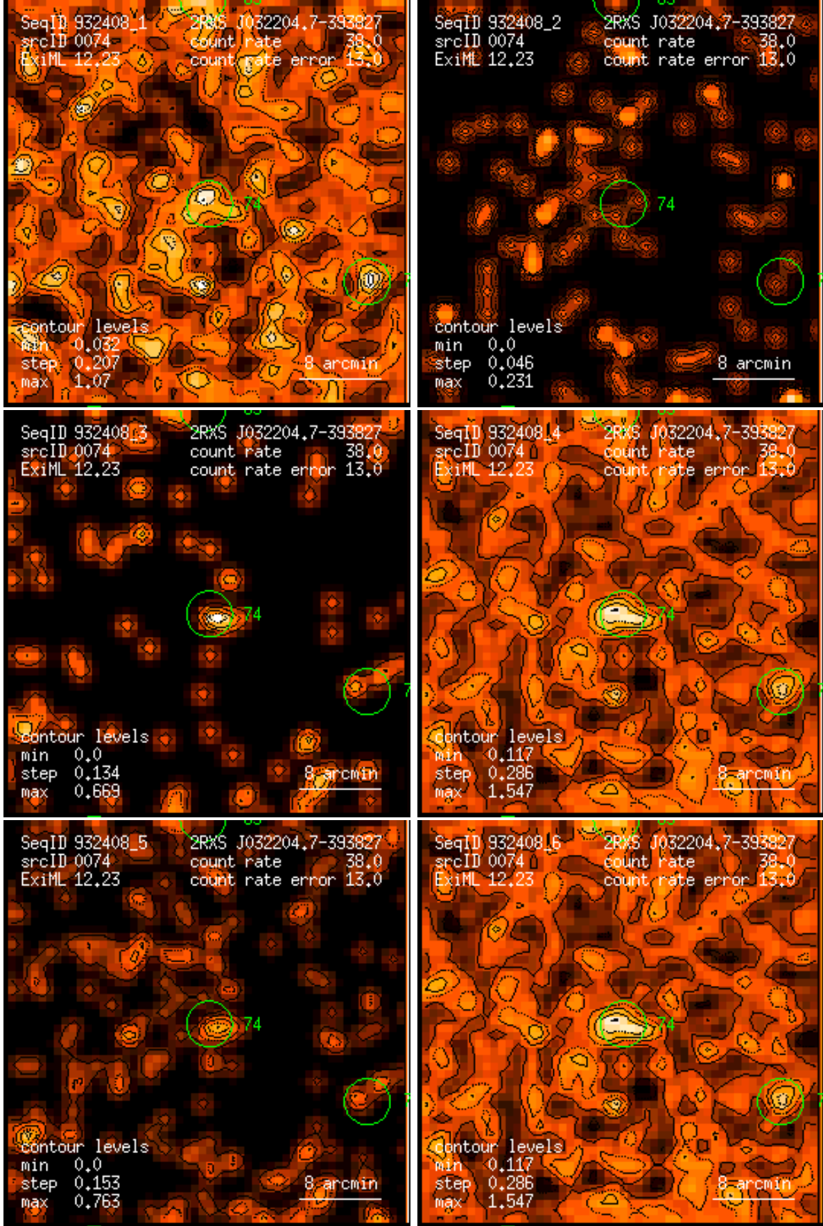
Figure 74: RASS 932408: detection 0074: band rate images, Gaussian filter: (1) PSPC channels 11 – 41, (2) 52 – 90, (3) 91 – 201, (4) 11 – 235, (5) 52 – 201, (6) 11 – 201. Broad band rates in counts/ks. Band rate contour levels in counts/ks/arcmin 2 .
